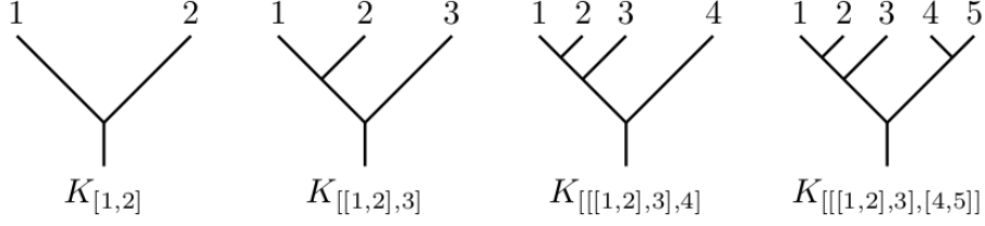
Fig. 7 Examples of the mapping between cubic graphs with one leg off-shell and BRST blocks. Together with the conventions (A.1), the fact that the BRST blocks furnish an explicit representation of the “Jacobi identity of trees” of the type discussed in [23] becomes manifest.
