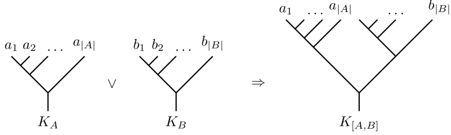
Fig. 8 The grafting operation on trees and its corresponding mapping in terms of BRST blocks.
