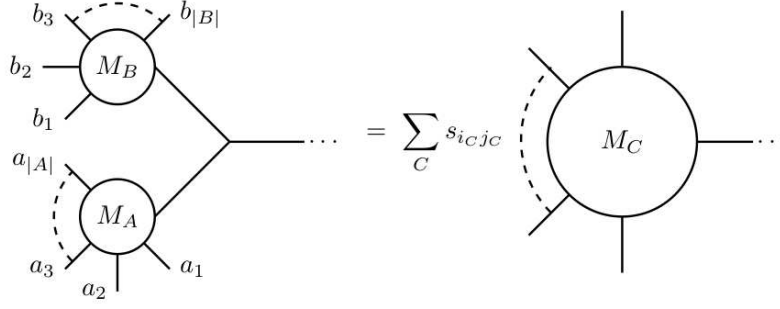
Fig. 10 Diagrammatic interpretation of M_{S[A,B]} .
