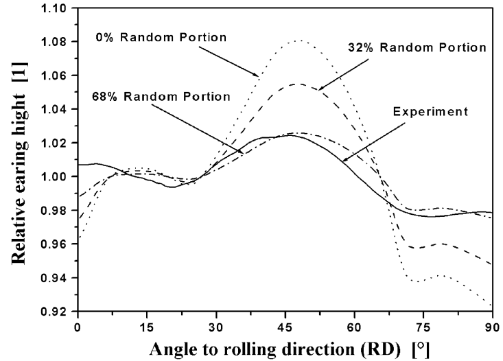
Fig. 10. Simulation and experimental results for earing in an aluminum sample the texture of which was approximated using two rolling texture components and a random texture component. The use of the fitted random background of 32 vol.% does not yield a satisfactory result in the finite element prediction. In order to achieve a good correspondence between simulation and experiment a value of 68% random had to be used.
