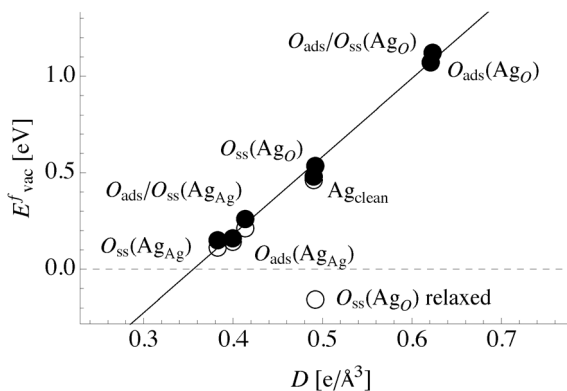
Fig. 13 Ag(111) surface vacancy formation energy in the presence of different oxygen species against the total directionality of the bond paths terminating at the associated surface atom. The filled (unfilled) circles represent unrelaxed (relaxed) vacancy formation energies.
