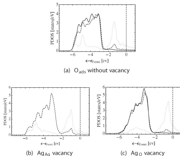
Fig. 6 PDOS on the surface silver and oxygen in the \text{O}_{\text{ads}} system. The \text{Ag}_{\text{Ag}} d-states are shown using solid lines, the \text{Ag}_{\text{O}} d-states as dashed lines, and the O p-states as dotted blue lines. The system is shown without a surface vacancy (a), with a \text{Ag}_{\text{Ag}} vacancy (b), and with a \text{Ag}_{\text{O}} vacancy (c).
