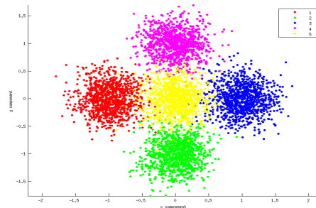
Fig. 6. Synthetic dataset with standard deviation 0.25.
