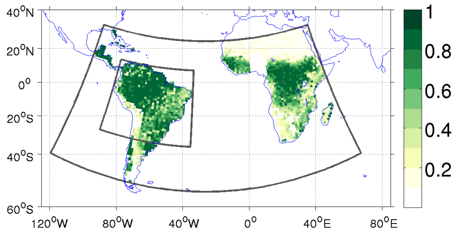
Figure 3. Land surface albedo (fraction) and locations of the coarse (140 km resolution) and nested (35 km resolution) domains for WRF-Chem simulations.
