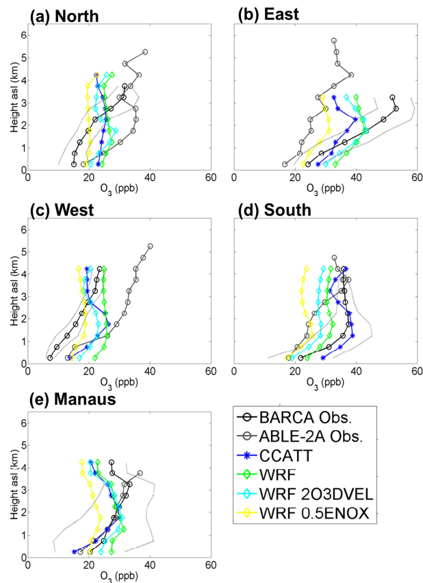
Figure 18. Mean vertical O 3 profiles for BARCA A flights for observations (black, gray line denotes one standard deviation), CCATT-BRAMS (blue) and WRF-Chem (base case – green, 2DEPVEL – cyan and 0.5ENox – yellow) simulations by region: (a) north, (b) east, (c) west, (d) south, and (e) around Manaus. ABL-2A observations (gray) from the same regions are included for comparison.
