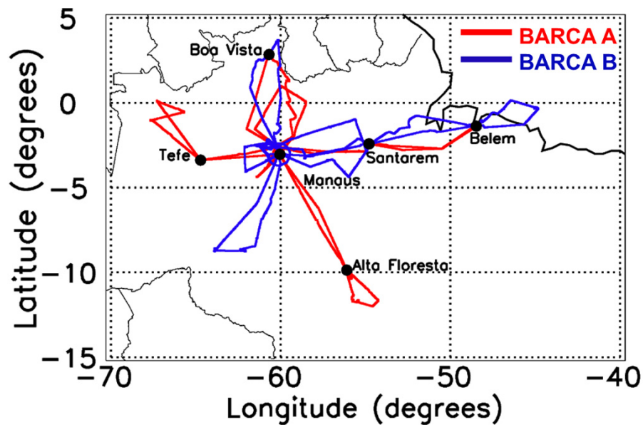
Figure 1. Flight tracks during BARCA.
