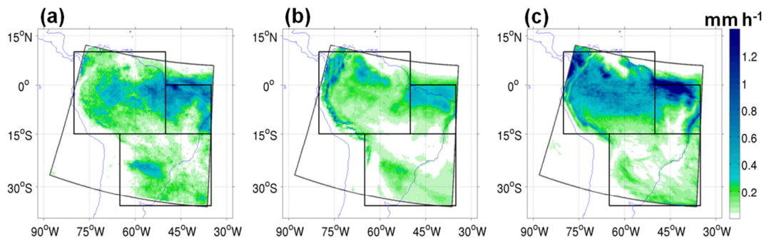
Figure 5. Same as Fig. 4, but for May 2009.
