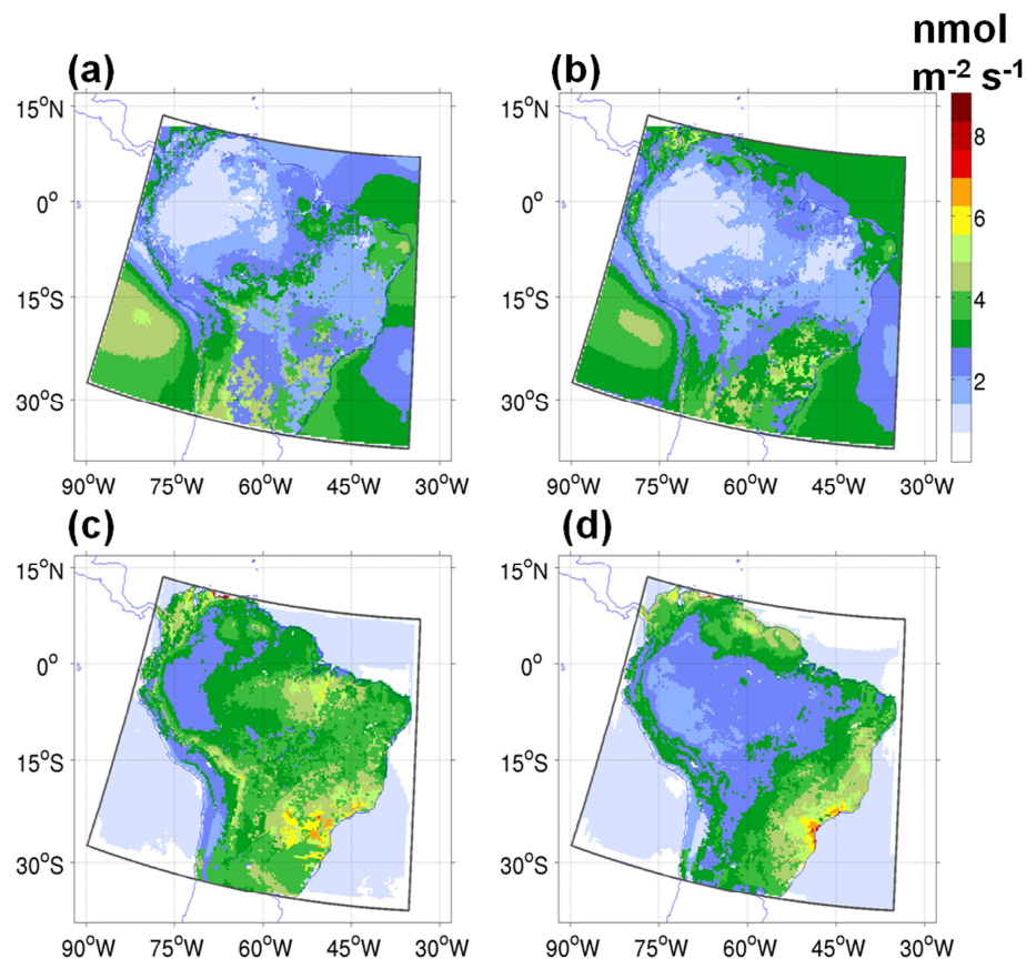
Figure 13. Average \text{O}_3 dry deposition flux ( \text{nmol m}^{-2} \text{s}^{-1} ) as simulated on the 35 km resolution domain (dark gray outline) by the CCATT-BRAMS model for (a) November 2008 and (b) May 2009 and by the WRF-Chem model for (c) November 2008 and (d) May 2009.
