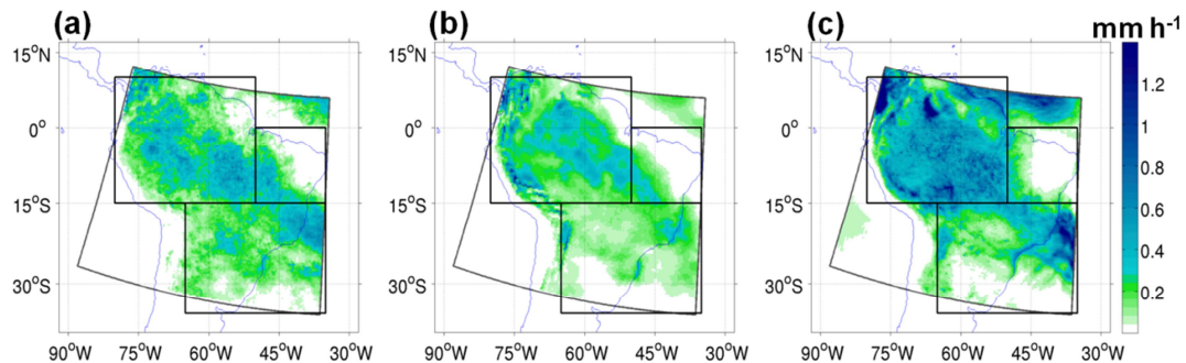
Figure 4. Monthly mean precipitation ( \text{mm h}^{-1} ) for November 2008 on the 35 km resolution domain (dark gray line) from (a) TRMM 3B43, (b) CCATT-BRAMS and (c) WRF-Chem. The subregions for precipitation comparison are indicated by black lines.
