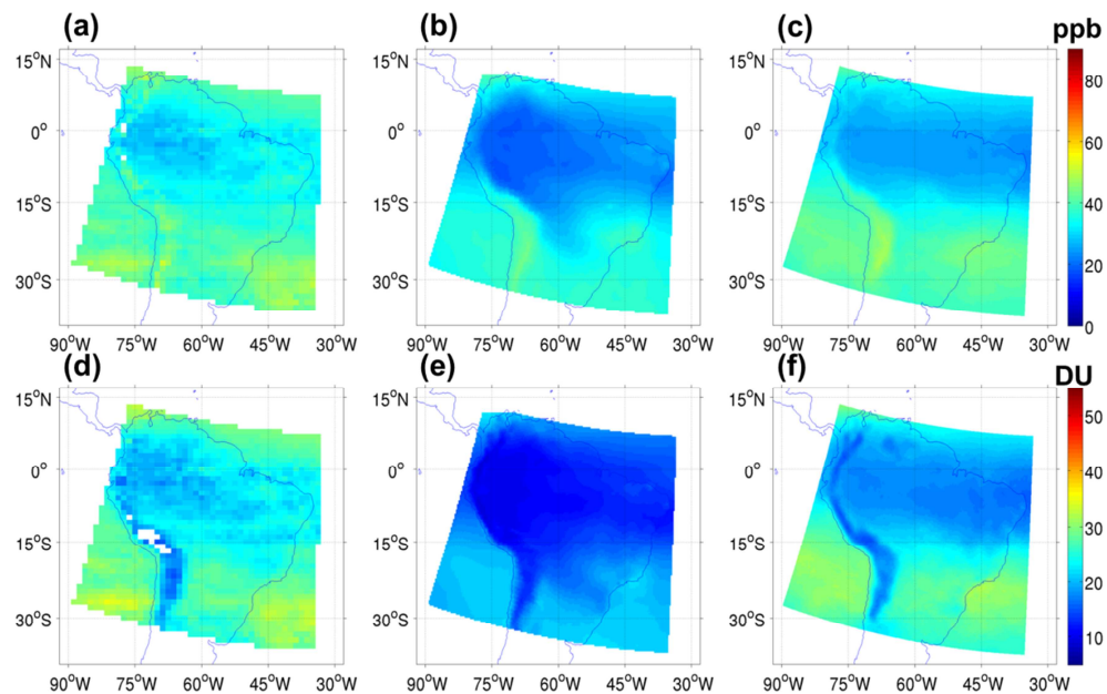
Figure 16. Same as Fig. 15, but for May 2009.
