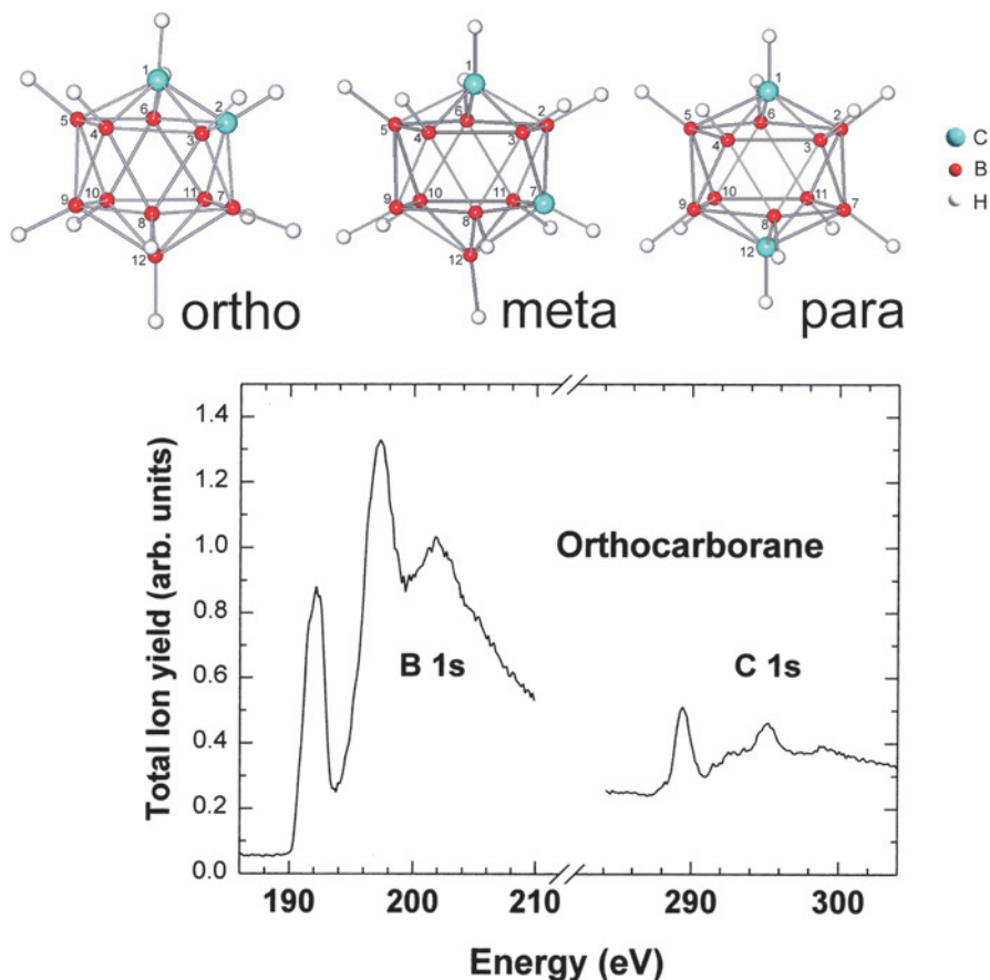
Figure 1: Schematic diagrams of the three isomers of closo - C_2B_{10}H_{12} , i.e. orthocarborane, metacarborane, paracarborane, with the total ion yield as a function of photon energy shown in the spectrum below for orthocarborane ( closo -1,2-dicarbododecaborane or 1,2- C_2B_{10}H_{12} ) at the B 1s and C 1s thresholds. Adapted from [1] and [3], with permission. For the other isomer total ion yields see [9].
