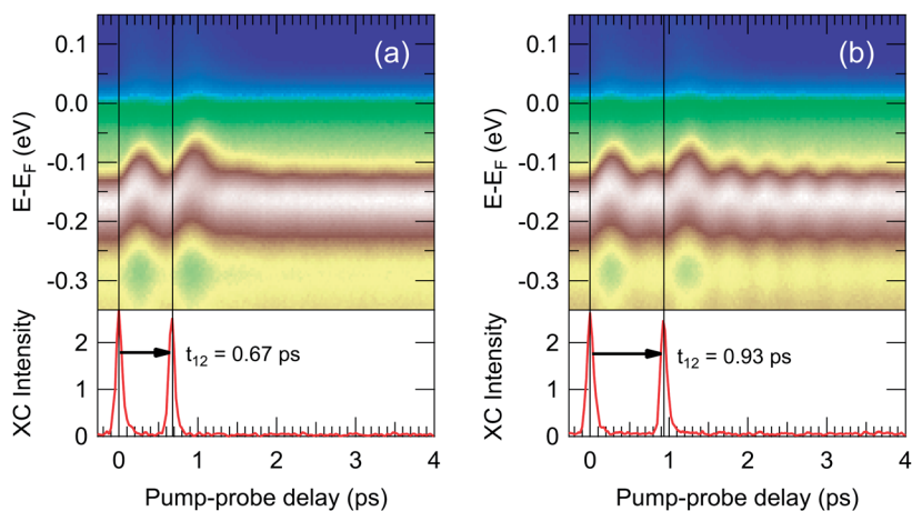
Fig. 5 (a) trARPES intensity of DyTe 3 at (k_x, k_y) \approx (0.13, 0.33)\text{\AA}^{-1} for a pump-pulse separation t_{12} = 0.67 ps, corresponding to a coherent quench of the amplitude mode oscillation (out-of-phase). The lower panel shows the cross correlation (XC) trace of the two pump pulses with the probe pulse obtained from electrons with E - E_F > 1.3 eV. (b) trARPES intensity for a pump-pulse separation t_{12} = 0.93 ps, corresponding to a coherent enhancement of the amplitude mode oscillation (in-phase).
