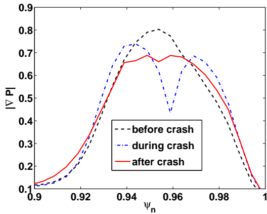
FIG. 4: Pedestal pressure gradient normalized over flux surfaces before (dash line), during (dash-dot line) and after (full line) the ELM crash.
