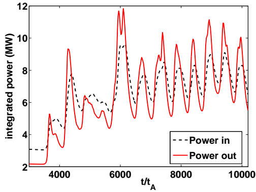
FIG. 6: Integrated power reaching the inner (dash line) and outer (full line) divertor plates.
