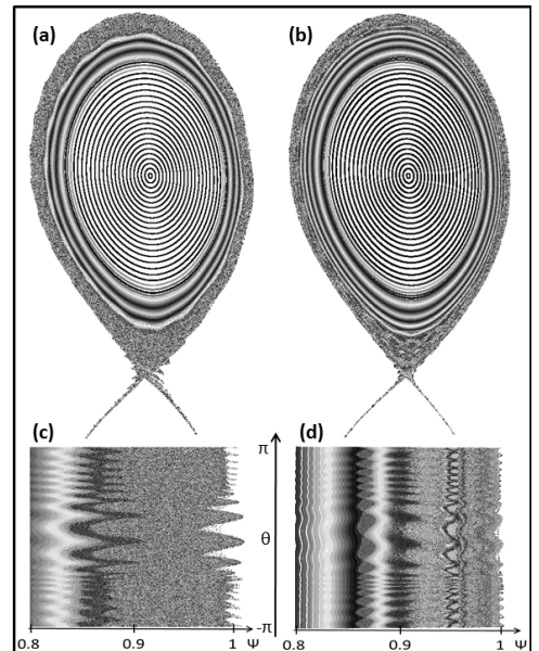
FIG. 2: Magnetic field topology in the n = 8 ELM simulation without diamagnetic effect, given at the peak of the ELM crash (a-c) and after the ELM crash at t \sim 7 \times 10^3 t_A (b-d). The figures (a) and (b) show the magnetic topology in the poloidal plane, and the figure (c) [respectively (d)] is a zoom of the plasma edge of the figure (a) [respectively (b)] in (\psi, \theta) coordinates for a normalized flux \psi \geq 0.8 . Note the full edge reconnection at the peak of the crash, and the remaining partial reconnection after the crash.
