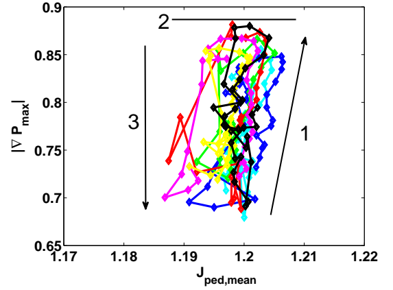
FIG. 5: Peeling-Ballooning diagram: evolution of the pressure gradient as a function of the mean pedestal current in quasi-periodic regime. The time between two points is 20t_A , and each color represents one ELM.
