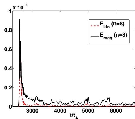
FIG. 1: Magnetic and kinetic energies of the mode n = 8 without diamagnetic effects. The time in x-axis is normalized to the Alfvén time t_A .
