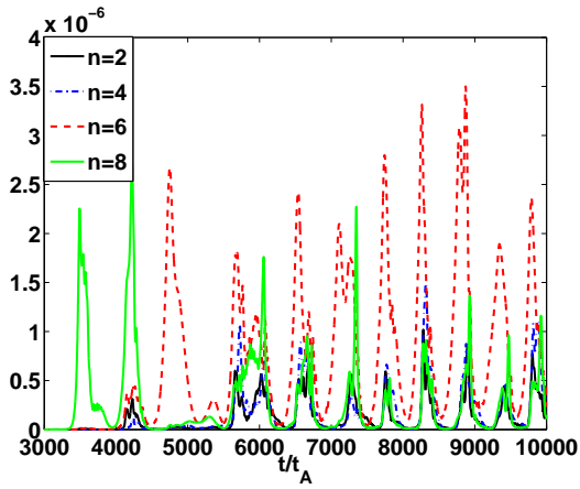
FIG. 3: Kinetic energy of the modes n = 2 - 8 in the multi-harmonic n = 0 : 2 : 8 simulation with diamagnetic effects.
