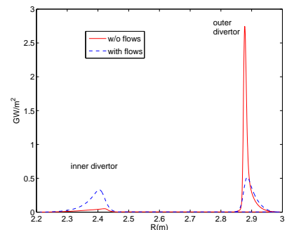
FIG. 7: Radial distribution of the heat flux (in GW/m^2 ) reaching the inner and outer divertor target plates: without flows included in simulation (full line) or with diamagnetic, neoclassical and toroidal flows (dashed line).
