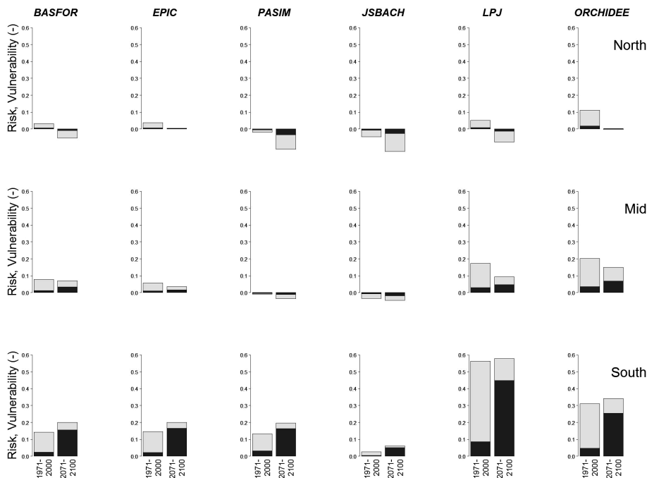
Figure 5. Drought risk analysis for NPP in two time periods (1971–2000, 2071–2100), for six different models. Top row: above 55° N, mid row: between 45 and 55° N, bottom row: below 45° N (see Fig. 3a). The whole bars depict vulnerability ( V ), the black parts are risks ( R ). V and R are expressed in relative terms, as fractions of NPP under non-hazardous conditions. Drought probabilities, P(H) , are equal to R/V .
