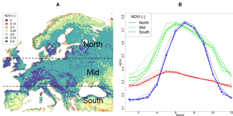
Figure 3. NDVI in Europe. (A) Average values of NDVI for April to September in 1982–2010. (B) Continuous lines: average monthly values of NDVI in the latitudinal bands delineated in (A) . The dashed lines are for years 2001–2005, the bold dashed line is for 2003.
