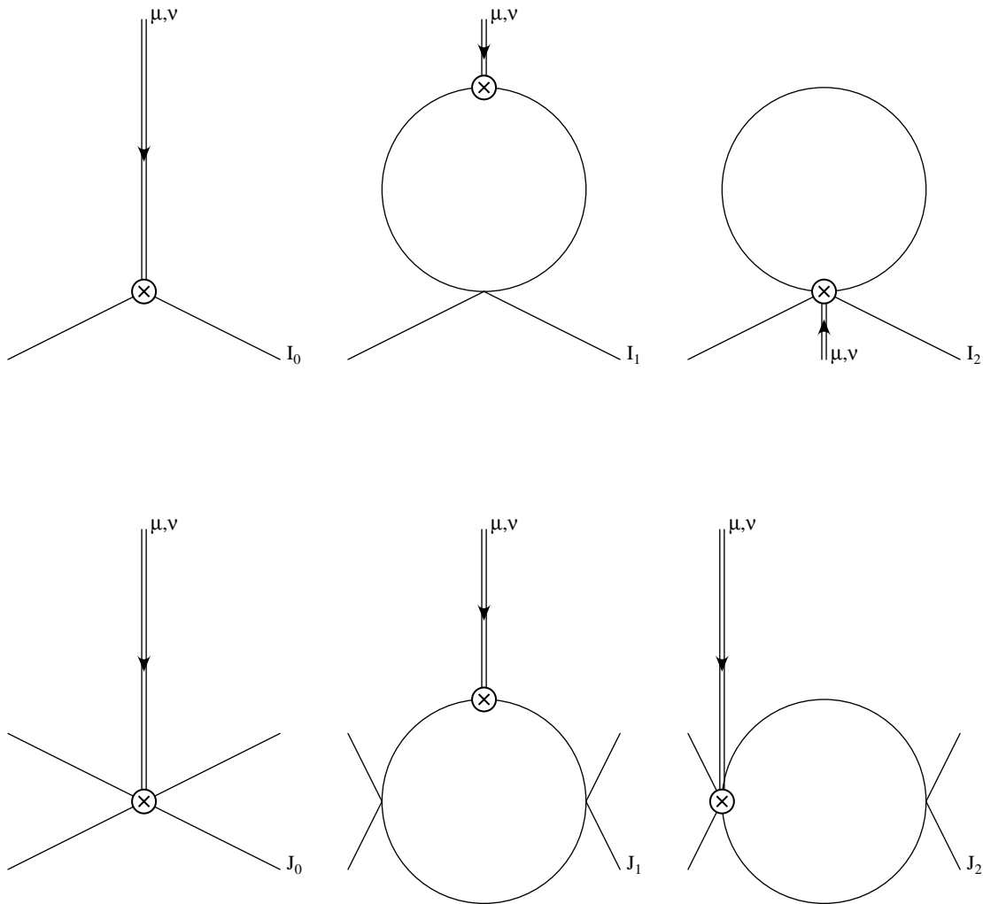
FIG. 1. The relevant insertions of T_{\mu\nu} .
