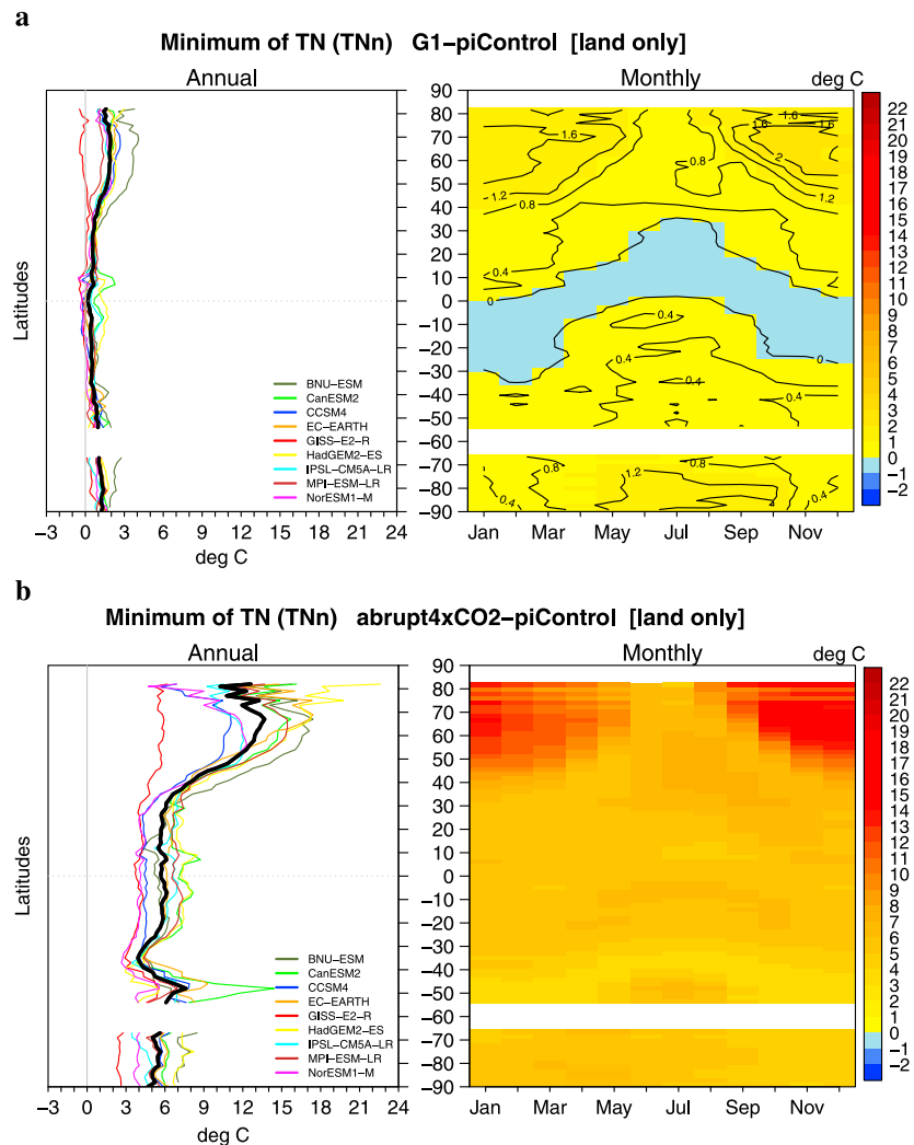
Figure 5. Multimodel, zonal mean (left column) annual and (right column) monthly anomalies in the extreme index TNn for the differenced experiments: (a) G1 - \pi Control and (b) abrupt4 \times CO_2 - \pi Control, taken over the fiducial 40 year analysis periods. Units are degrees Celsius in all panels. The zonal averages are computed over land points only, which accounts for the gaps in the Arctic and Antarctic oceans. An alternate version of Figure 5a showing the more detailed structure of the G1 - \pi Control differences is provided in supporting information Figure S5a.
