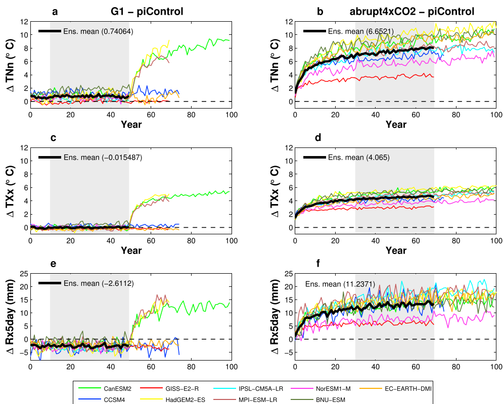
Figure 2. Time series of the difference of global mean extreme indices from piControl values for all models analyzed. Left-hand panels show the difference G1 - piControl , right-hand panels abrupt4 \times CO_2 - piControl , and the indices are, from top to bottom, TNn , TXx , and Rx5day . The heavy dark curve is the multimodel mean, and gray shading indicates the 40 year analysis period for each experiment used in this study. The values at the top left in each panel are the multimodel and time mean of the indicated index over the analysis period.
