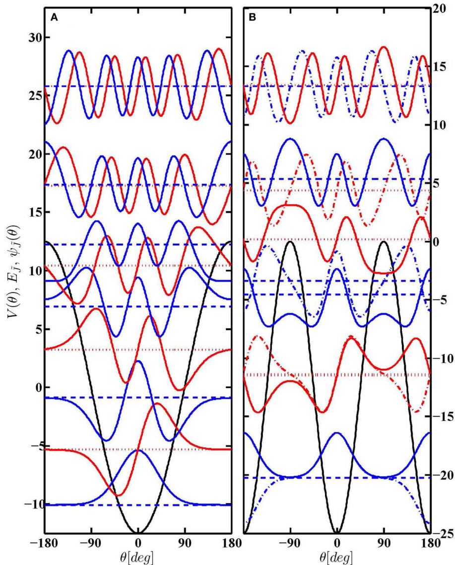
FIGURE 1 | Eigenenergies and eigenfunctions pertaining to Hamiltonian of Equation (1). Left panel (A): purely orienting interaction with \eta = 12.5 , \zeta = 0 . Right panel (B): purely aligning interaction with \eta = 0 , \zeta = 25 , where the tunneling doublets can be understood as
