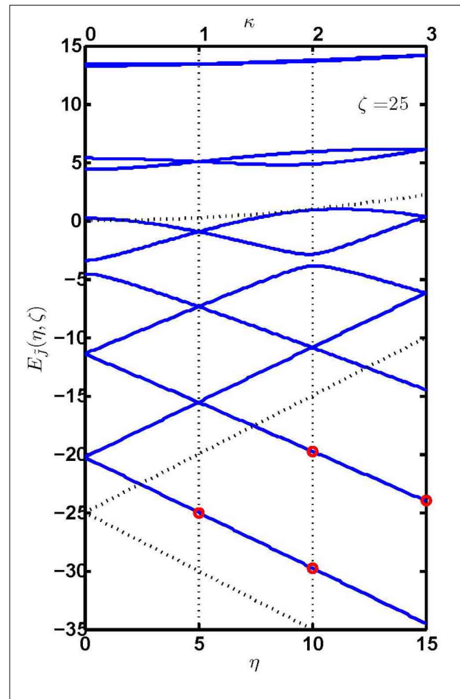
FIGURE 4 | Eigenenergies of a planar rotor subject to the combined orienting and aligning interactions as a function of \eta for a fixed \zeta = 25 .
