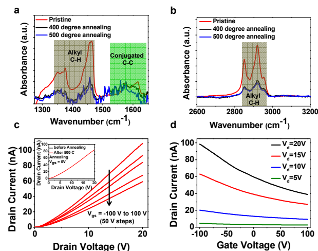
Figure 3. a, b) ATR-FTIR normalized spectra of pristine, 400 and 500\text{ }^{\circ}\text{C} annealed GNR films showing relative intensity decrease in peaks associated with alkyl C-H bonds for annealed samples. c) current vs. drain voltage ( I - V_d ) of a typical GNR film device under different gate voltages ( V_{gs} ). d) current vs. gate voltage ( I - V_{gs} ) of the same device under dif-
