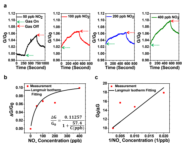
Figure 4. \text{NO}_2 gas sensing experiment using a GNR film device. a) Time domain normalized conductance ( G/G_0 ) of the GNR film device whilst introducing different concentrations of \text{NO}_2 . Green arrows correspond to the device being exposed to a certain concentration of \text{NO}_2 while red arrows correspond to the device being flushed with Ar only. b) Measured conductance change ( \Delta G/G_0 ) of the device in (a) as a function of \text{NO}_2 concentration (red squares) and the corresponding Langmuir isotherm curve fitting (black line). Langmuir isotherm fitted equation is written in bottom right
