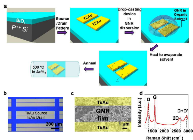
Figure 2. a) Scheme of GNR film device fabrication. b) Optical image of the fabricated devices. c) SEM image of a typical GNR film device with GNR films between two (falsely colored)
