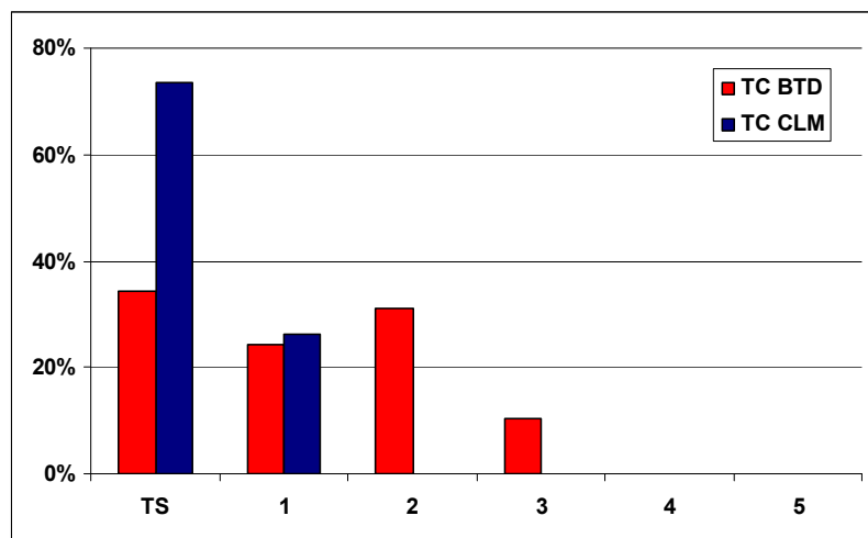
Figure 4.11 Distribution of TCs in the CCLM-SN ensemble mean (blue) and in BTDO observations (red) sorted by SSHS intensity categories, based on TC lifetime maximum wind speed. The x-axis shows SSHS categories extended by tropical storm category.
