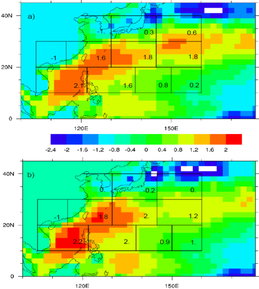
Figure 5.5 First pair of canonical correlation patterns derived between regional time series of TC occurrences anomalies (CCA TC) and fields of sea surface temperature anomalies (CCA SST). Sea surface temperature fields are provided by NCEP reanalysis. TC fields are derived from a) BTM observations, sharing a CCA correlation of 59 % b) CCLM, sharing a CCA correlation of 58 %. CCA SST is shaded, CCA TC coefficients are given as numbers in each corresponding subregion.
