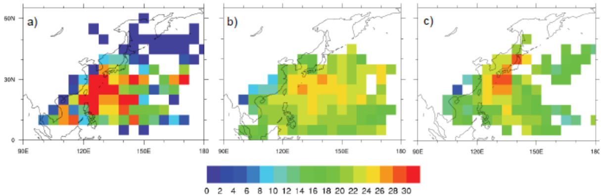
Figure 4.7 TC mean wind speed spatial distribution (TC wind speed cumulated within 5^\circ latitude \times 5^\circ longitude grid boxes; normalized by the mean TC spatial density) for a) BTD; b) CCLM-NN; c) CCLM-SN. Gridboxes where TC occurred less than 3 times are not shaded.
