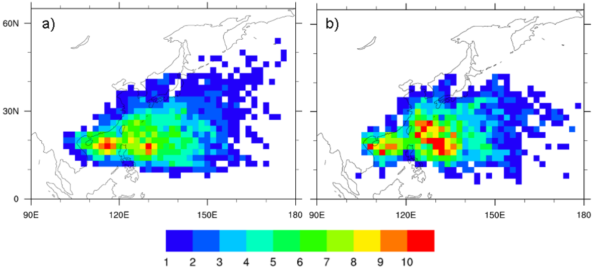
Figure 5.1 TC spatial densities (accumulated TC occurrence per every 2° latitude x 2° longitude grid box; normalized by the mean spatial density fields) for a) BTM, b) CCLM in the period 1978-2011.
