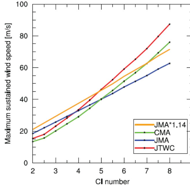
Figure 3.3 Relationship of Current Intensity parameter to maximum sustained 10 m wind speed [ \text{m s}^{-1} ] using conversion tables used in JTWC (Dvorak), JMA (Koba), JMA*1.14 (Koba multiplied by a factor of 1.14), CMA (Dvorak multiplied by a factor of 0.87). The x-axis shows the Current Intensity numbers, while the y-axis shows wind speed [ \text{m s}^{-1} ].
