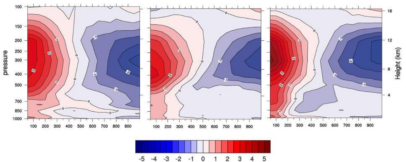
Figure 4.5 Vertical temperature anomalies [unit: K degrees] averaged over the radial distance from the TC centre for typhoon Songda at its stage with maximum near-surface wind speed for NCEP CFSR (left), and CCLM-NN (middle) and CCLM-SN (right) ensemble means. The x-axis shows the radial distance [unit: km]. The left y-axis shows pressure levels [unit: hPa], the right y-axis shows height [unit: km].
