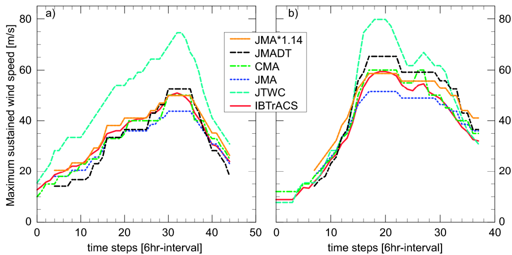
Figure 3.4 Wind speed time series for two TC events: a) Isa (1997), b) Dianmu (2004) for original BTD sets: JMA, CMA, JTWC, IBTrACS and modified BTD sets: JMA*1.14, (JMA multiplied by a factor), JMADT (JMA using the Dvorak conversion table). The x-axis shows time steps along the typhoon track, for which intensity in BTD sets was provided.
