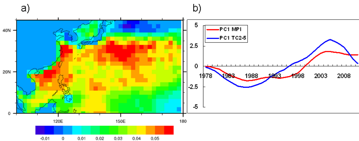
Figure 5.6 a) First EOF representing decadal variability of the Maximum Potential Intensity in CCLM. b) EOF time series for: Maximum Potential Intensity (PC1 MPI, red) and TC-days number for the intense TCs (PC1 TC2-5, blue). Time series share a correlation of 91 %. The x-axis shows years from the period 1978-2011.
