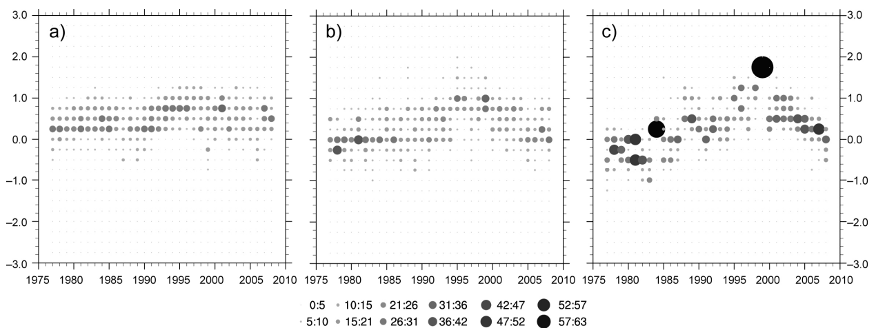
Figure 3.5 Yearly distributions of Current Intensity number differences for JTWC- JMADT assigned to intensity categories: a) tropical depression, tropical storm, 1, b) 2-3, c) 4-5. The x-axis shows years, while the y-axis shows Current Intensity difference. The size of the circles indicates the percentage of the occurrence number, counted for each year separately.
