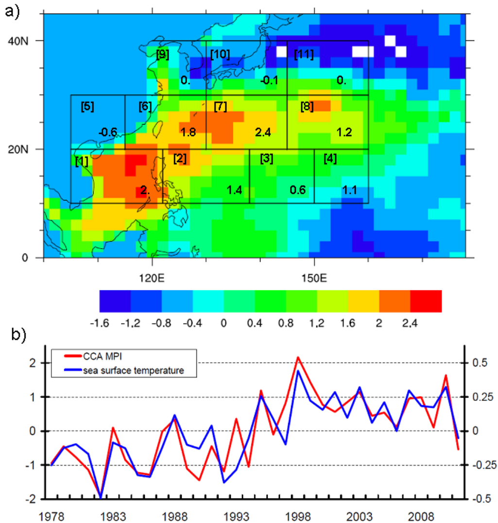
Figure 5.4 a) The first pair of canonical correlation patterns – derived between regional time series of TC occurrences anomalies (CCA TC) and fields of maximum potential intensity anomalies (CCA MPI). CCA pair shares a correlation of 71 % for the period 1978-2011. CCA MPI is color - shaded, CCA TC coefficients are given as numbers in each corresponding subregion. The number of the region is given in brackets. b) Time series of canonical coefficients of maximum potential intensity anomalies (CCA MPI, red) sharing a correlation of 85 % with mean sea surface temperature anomalies (blue) over the main TC genesis area in the WNP (100°E - 180°E, 5-30°N). The left y-axis shows canonical coefficients, the right y-axis corresponds to the sea surface temperature anomalies. The x-axis shows years from the period 1978-2011.
