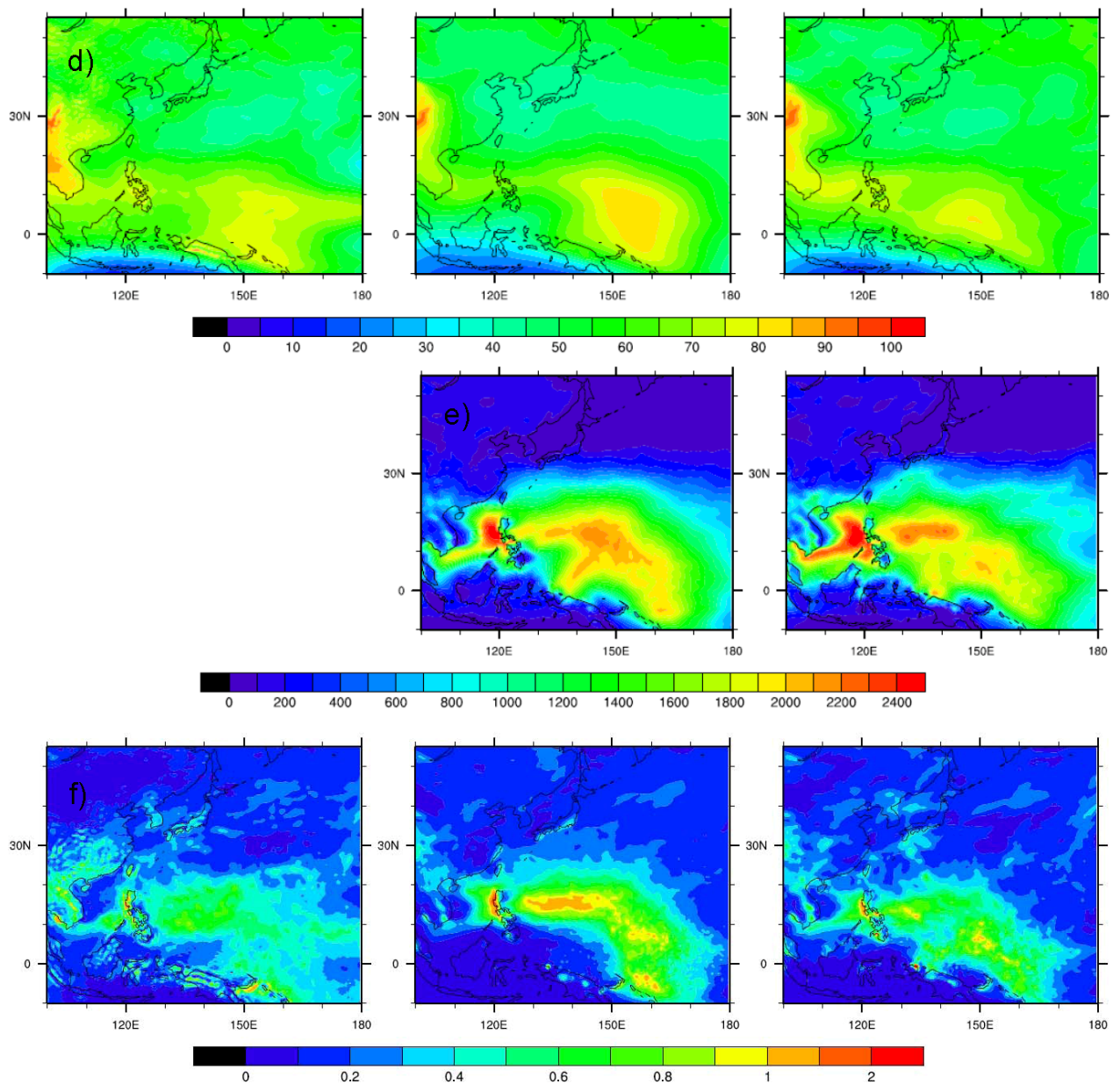
Figure 4.8 cd.: d) relative humidity on 600 hPa [unit: mm], e) convective available potential energy [unit: J kg^{-1} ], f) hourly precipitation [unit: mm] in CFSR (left column) CCLM-NN ensemble mean (middle column) and CCLM-SN ensemble mean (right column). Convective available potential energy is not provided by CFSR, therefore it is shown only for CCLM-NN and CCLM-SN.
