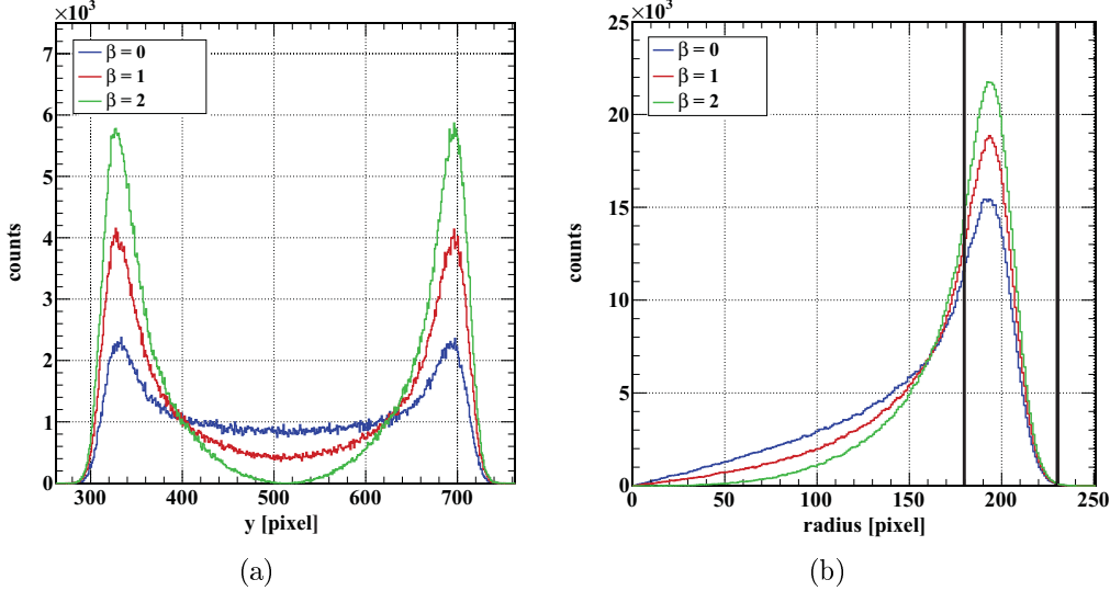
Figure 6.2: (a) Cuts parallel to the y axis through the center of the images in Fig. 6.1. (b) Radial projections of the images in Fig. 6.1, see also section 3.2.4. The simulated electron kinetic energy has a Gaussian distribution centered at r = 200 pixels with a width of \sigma_r = 5 pixels.
