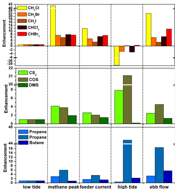
Figure 4. Relative enhancement of selected VOC fluxes from a tidally influenced seagrass bed. All fluxes were normalized to the respective mean fluxes during low tide. \text{CS}_2 , \text{CH}_3\text{Cl} , \text{CH}_3\text{Br} , \text{CH}_3\text{I} , \text{CHCl}_3 , \text{CHBr}_3 , and propene were quantified against a Scott TOC 15/17 standard. Relative fluxes for \text{COS} , propane, butane and \text{DMS} were calculated from the measured intensities. For clarity the variability of the VOC fluxes is not shown. Mean and ranges are provided in Table 2.
