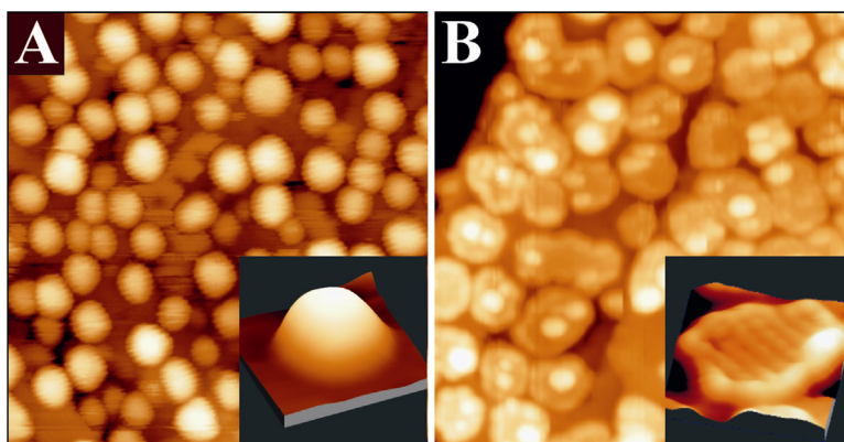
Fig. 6. STM images of 0.7 mL Au dosed onto (a) pristine and (b) doped CaO films (4.5 V, 50 nm × 50 nm). The insets display close-ups of two characteristic particles (−5.0 V, 10 nm × 10 nm) [42].
