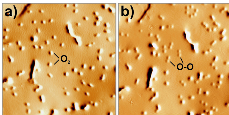
Fig. 8. STM images of the same O 2 -covered region of Mo-doped CaO taken (a) before and (b) after multiple scans at 4.0 V (3.3 V, 40 nm × 40 nm). Note the dissociation of most molecules into atom pairs upon electron injection from the tip. While atoms appear with pronounced sombrero shapes at higher bias, the molecules are imaged as deep depressions in the surface [9].
