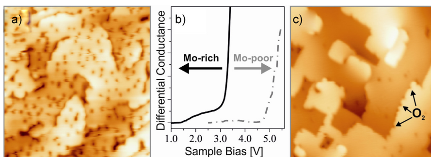
Fig. 7. (a and c) STM images of strongly and weakly doped CaO films after exposure to 5 L O 2 @ 20 K (40 nm × 40 nm). The O 2 adsorption probability correlates with the position of the CaO conduction band, as measured with dI/dV spectroscopy (b) Step edges are preferred O 2 binding sites only on weakly doped films (see arrows in c) [9].
