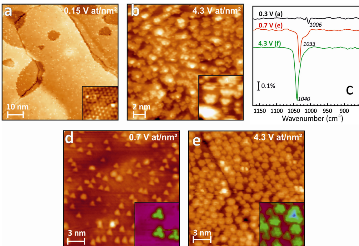
Fig. 2. (a and b) STM images of \text{VO}_x deposited on \text{CeO}_2(111) thin films in oxygen at 300 K with vanadia coverages of 0.15 at/nm 2 (a), and 4.3 at/nm 2 (b). STM images of samples (b) after annealing to 700 K are shown in (d) and (e), respectively. Insets show high-resolution images of the vanadia species such as monomers, dimers, trimers, and heptamers. IR-spectra of the samples imaged in (a) and (d) and (e) are shown in (c) [2,3].
