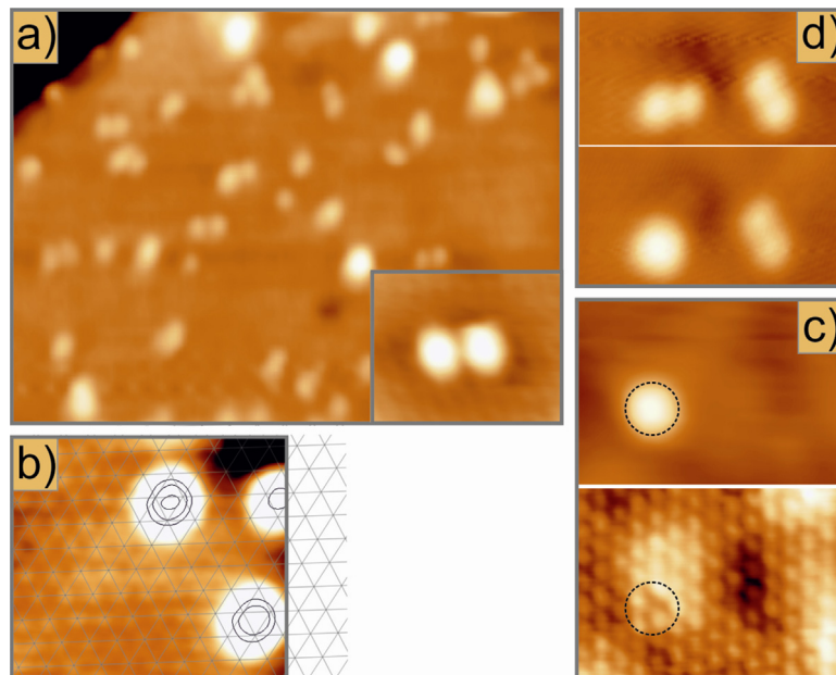
Fig. 5. (a) Ceria surface after dosing 0.05 \text{ mL} of Au at 10 \text{ K} ( 2.5 \text{ V} , 26 \text{ nm} \times 20 \text{ nm} ). Note the abundance of atom pairs on the surface. The pair in the inset shows a pronounced sombrero shape, indicating its charged nature. (b) STM image showing the Ce sub-lattice and three Au atoms bound to regular O-top sites. (c) Au adatom bound to a subsurface defect, as deduced from the atomically resolved image taken after atom removal with the tip (both 4.2 \text{ nm} \times 3.0 \text{ nm} ). (d) Transformation of an Au atom pair into an upright standing dimer via a tip-voltage pulse ( 5.5 \text{ nm} \times 3.0 \text{ nm} ) [37].
