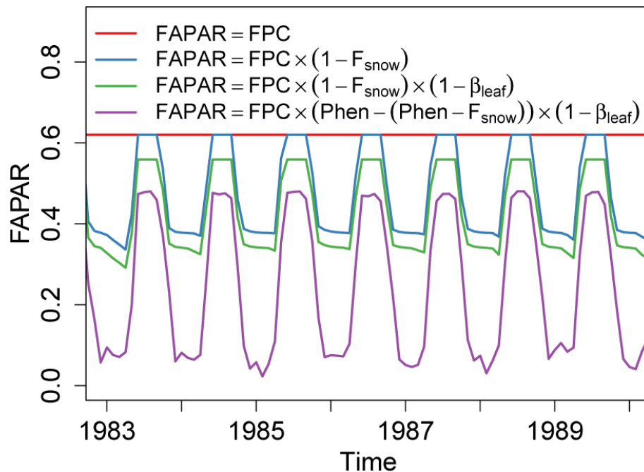
Figure A1. Effects on FAPAR in LPJmL for an example grid cell in Siberia. FAPAR in LPJmL is computed from foliar projective cover (FPC), from snow coverage in the green canopy ( F_{\text{snow}} ), leaf albedo ( \beta_{\text{leaf}} ) and phenology status (Phen).
