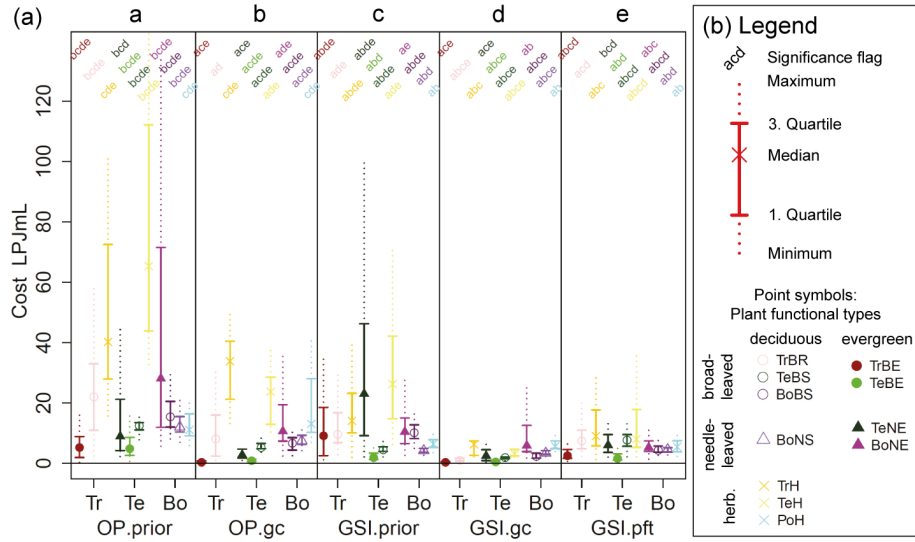
Figure D2. Distribution of the cost for several grid cells in prior model runs and optimization experiments grouped by plant functional types and biomes. (a) Cost for LPJmL-OP with default parameters ( a , OP.prior), after grid cell-level optimizations ( b , OP.gc), cost for LPJmL-GSI with prior parameters ( c , GSI.prior), after grid cell-level optimizations ( d , GSI.gc) and after PFT-level optimizations ( e , GSI.pft). Biomes are Tr (tropical), Te (temperate) and Bo (boreal/polar). (b) Legend for the plot. Each distribution is plotted according to usual boxplot statistics. The point symbols indicate the plant functional type. The significance flag on top of each distribution shows if a distribution is significant different ( p \leq 0.01 ) to the corresponding distribution of the same PFT in another optimization experiment. The significance is based on the Wilcoxon rank-sum test. For example “acd” indicates a significant difference to the corresponding categories (a) (OP.prior), (c) (GSI.prior) and (d) (GSI.gc) but no significant difference to (b) (OP.gc) and (e) (GSI.pft).
