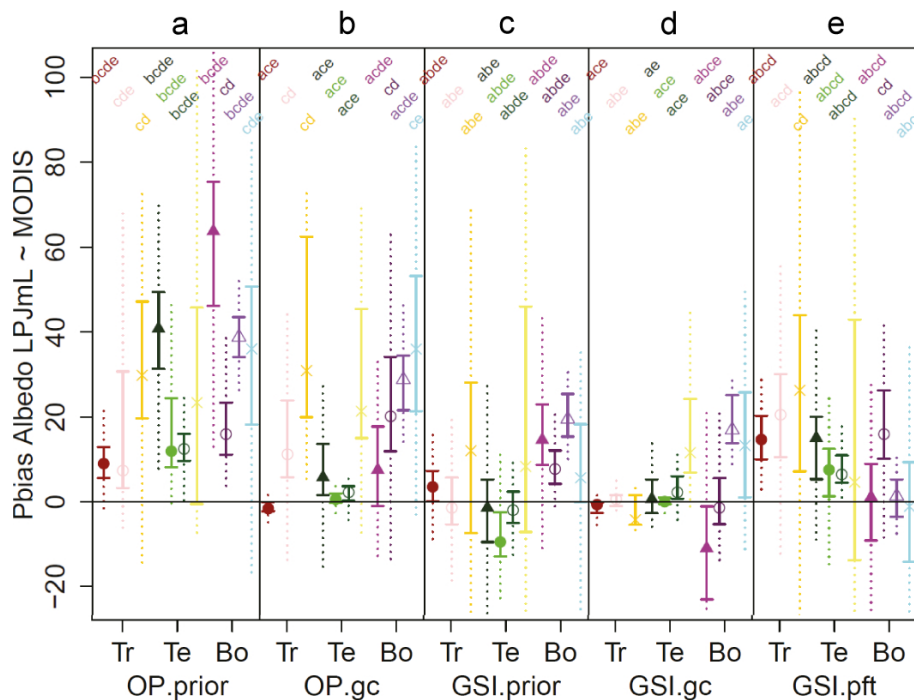
Figure D4. Distribution of the percent bias between LPJmL and MODIS monthly growing season albedo (2000–2011) for several grid cells in prior model runs and optimization experiments grouped by plant functional types and biomes. See Fig. D2 for a further explanation of this figure.
