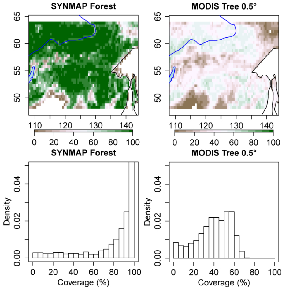
Figure C2. Comparison of total forest coverage from SYNMAP and MODIS tree coverage for a region in eastern Siberia.
