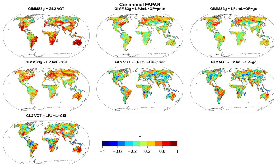
Figure E5. Correlation coefficients between annual FAPAR time series (annual mean averaged from monthly values with air temperatures > 0^{\circ}\text{C} ) from GIMMS3g, GL2 VGT datasets and LPJmL model simulations.
