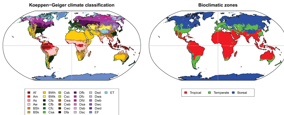
Figure C1. Reclassification of the Koeppen–Geiger climate classification in bioclimatic zones.
