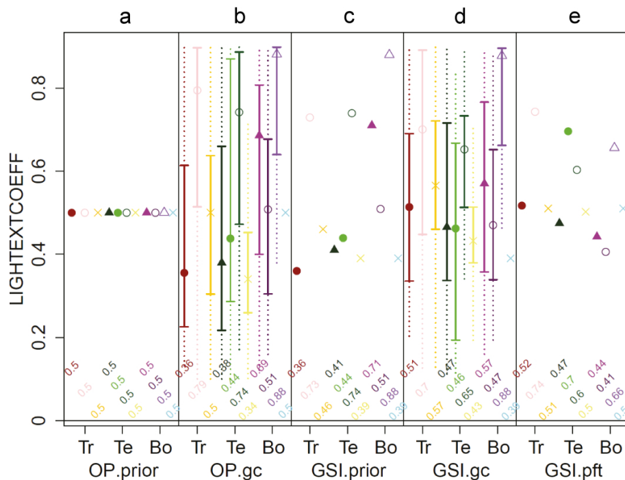
Figure D7. Prior and optimized values for the parameter k (light extinction coefficient) grouped by plant functional types and biomes. The distribution of the parameter in the optimization experiments OP.gc and GSI.gc represents the spatial variability of the parameter from different grid cell-level optimization experiments. See Fig. D2 for a further explanation of this figure.
