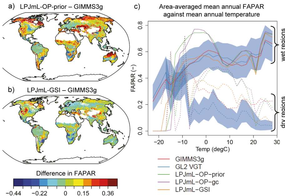
Figure 7. Comparison of mean annual FAPAR from LPJmL and remote sensing datasets. (a) Difference in mean annual FAPAR between LPJmL-OP-prior and GIMMS3g. (b) Difference in mean annual FAPAR between LPJmL-GSI and GIMMS3g. (c) Global spatial-averaged gradients of mean annual FAPAR from LPJmL and data sets. The uncertainty of the GL2 VGT FAPAR dataset is shown as blue area. Dashed lines are dry regions with mean annual P/PET < 15 and solid lines are wet regions with mean annual P/PET \geq 15 .
