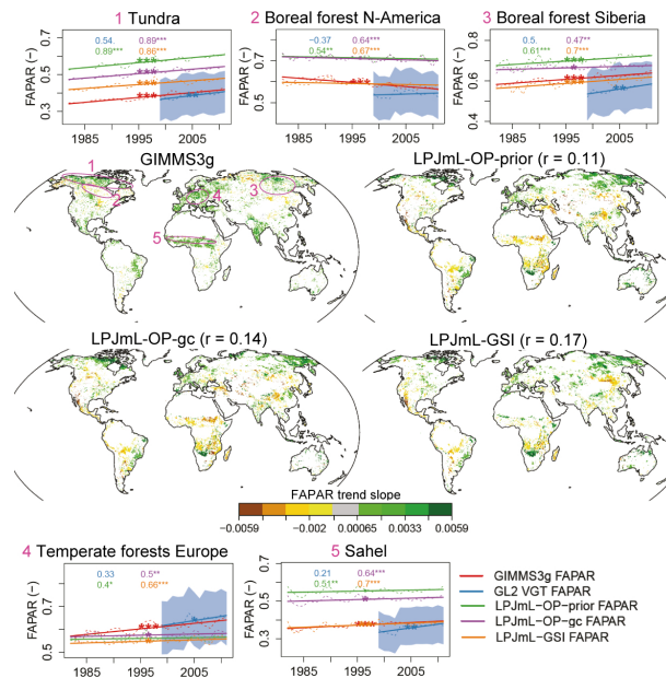
Figure 11. Comparison of trends in mean annual FAPAR from LPJmL and from satellite datasets. Trends were computed between 1982 and 2011 as linear trends. The significance of a trend was determined using the Mann–Kendall trend test. Only significant trends slopes ( p \leq 0.05 ) are displayed in each map. Spatial correlations of trend slopes (Spearman coefficient) between LPJmL and the GIMMS3g dataset are given in the map titles. Time series are showing mean annual FAPAR time series and trends spatially averaged for the regions as indicated in the first map. The blue area in time series represents the uncertainty of the GL2 VGT FAPAR dataset. Numbers in the time series plot are correlation coefficients between mean annual FAPAR time series from GIMMS3g and from GL2 or LPJmL model runs, respectively. The significance of a trend and of the correlation is indicated as point symbol: *** ( p \leq 0.001 ), ** ( p \leq 0.01 ), * ( p \leq 0.05 ), . ( p \leq 0.1 ).
