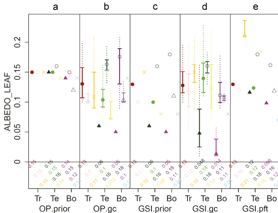
Figure D6. Prior and optimized values for the parameter \beta leaf (leaf albedo) grouped by plant functional types and biomes. The distribution of the parameter in the optimization experiments OP.gc and GSI.gc represents the spatial variability of the parameter from different grid cell-level optimization experiments. See Fig. D2 for a further explanation of this figure.
