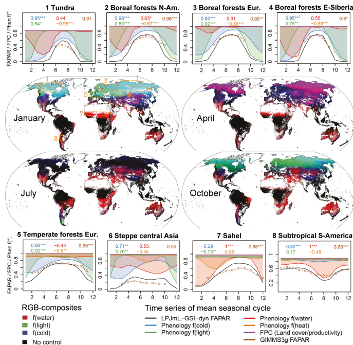
Figure 12. Phenological controls on seasonal FAPAR dynamics. The maps are red-green-blue composites of the mean monthly values for the water (red), light (green) and cold temperature (blue) phenology limiting function values from the LPJmL-GSI-dyn model run. White regions in the maps are without vegetation or dominated by croplands for which the LPJmL-GSI phenology model was not applied. Time series represent the mean seasonal cycles (January to December) (averaged over 1982–2011) of simulated and observed FAPAR and phenology limiting function values averaged for different regions as indicated in the first map. Phenology limiting function values close to 0 indicate a strong control by phenology limiting functions whereas values close to 1 indicate no phenological control. The correlation coefficients of each time series with the simulated FAPAR time series are shown in each time series plot. The significance of the correlation is indicated as point symbol: *** ( p \leq 0.001 ), ** ( p \leq 0.01 ), * ( p \leq 0.05 ), . ( p \leq 0.1 ).
