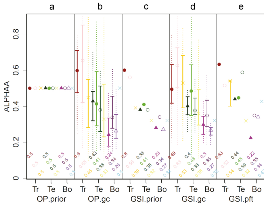
Figure D5. Prior and optimized values for the parameter \alpha (fraction of radiation absorbed at leaf level relative to canopy level) grouped by plant functional types and biomes. The distribution of the parameter in the optimization experiments OP.gc and GSI.gc represents the spatial variability of the parameter from different grid cell-level optimization experiments. See Fig. D2 for a further explanation of this figure.
