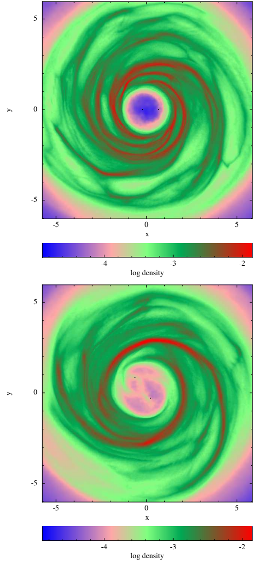
Figure 2. DISC SURFACE DENSITY OF RUNS retro \epsilon = 00 (TOP) AND retro \epsilon = 08 (BOTTOM) - Colors are in log-density scale as indicated by the colour-bars, all plots are in code units G = M_0 = a_0 = 1 and snapshots are taken at the same time t = 70 .
