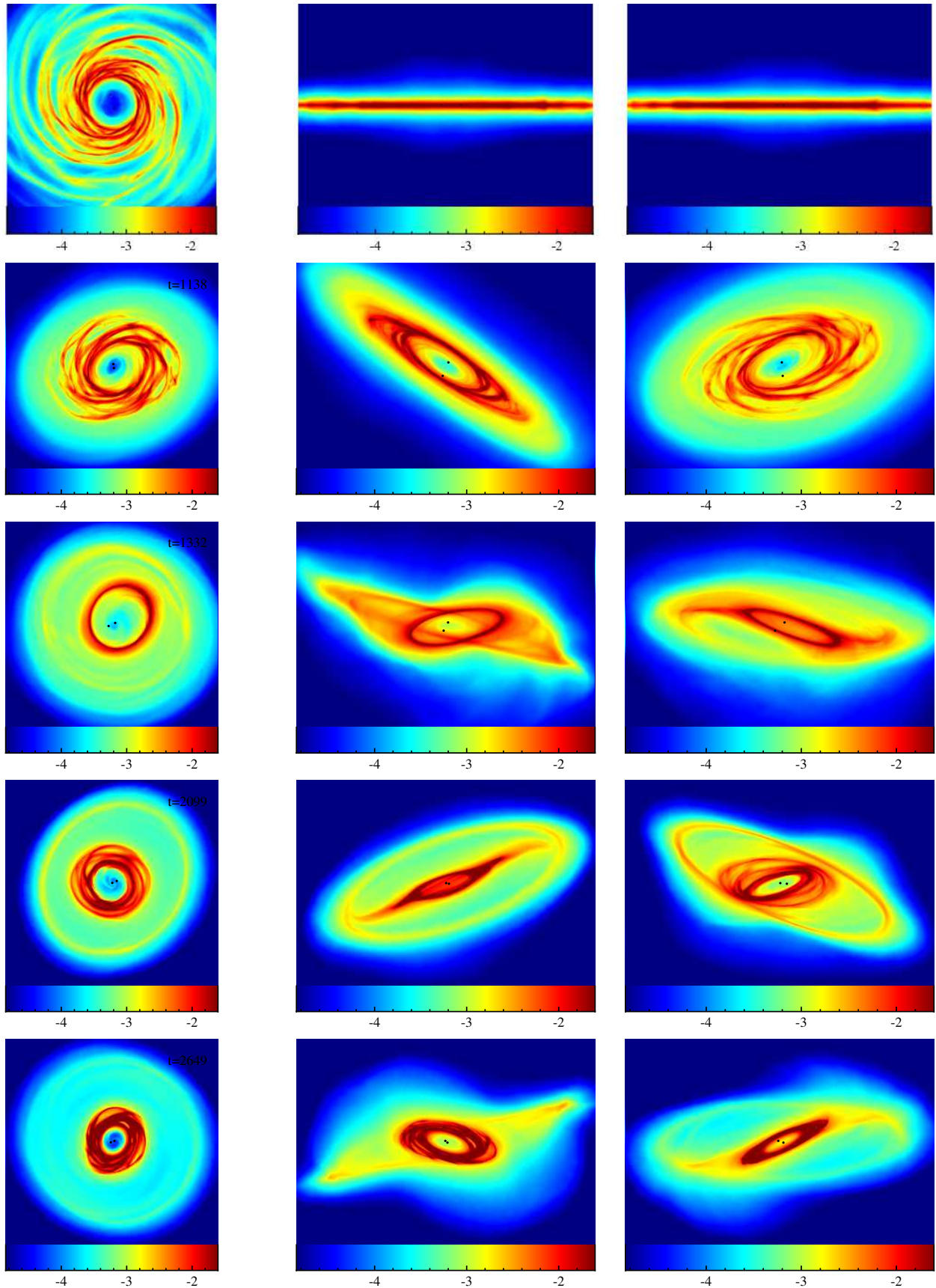
Figure 11. THE TILTING INSTABILITY: LOGARITHMIC COLUMN DENSITY, FACE-ON xy , EDGE-ON xz , EDGE-ON yz - Time evolution (top to bottom) of the high accuracy, tilting "retro" \epsilon = 0.9 " run. Panels show the successive stages of the binary first tilting out of plane and then subsequently aligning with the disc. Note the spread into various annuli that the disc undergoes in the middle panels.
