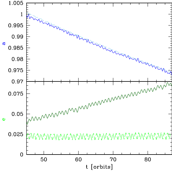
Figure 6. EVOLUTION OF SEMI MAJOR AXIS AND ECCENTRICITY FOR CIRCULAR BHBS - Direct comparison of the prograde (solid lines) and retrograde (dashed lines) systems. Only the stage after the initial transient is shown. The evolution of a cannot be distinguished between the two setups, whereas the evolution of e is substantially different.
