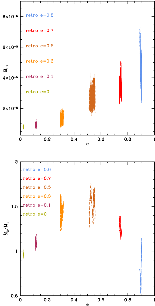
Figure 9. MASS TRANSFER RATES AS FUNCTION OF ECCENTRICITY - ( Top ): Total accretion rate for the different runs. ( Bottom ): ratio between secondary and primary accretion rate \dot{M}_2/\dot{M}_1 , as a function of eccentricity for the retrograde runs. All retro runs are plotted over the same time interval (orbits 45 – 90).
