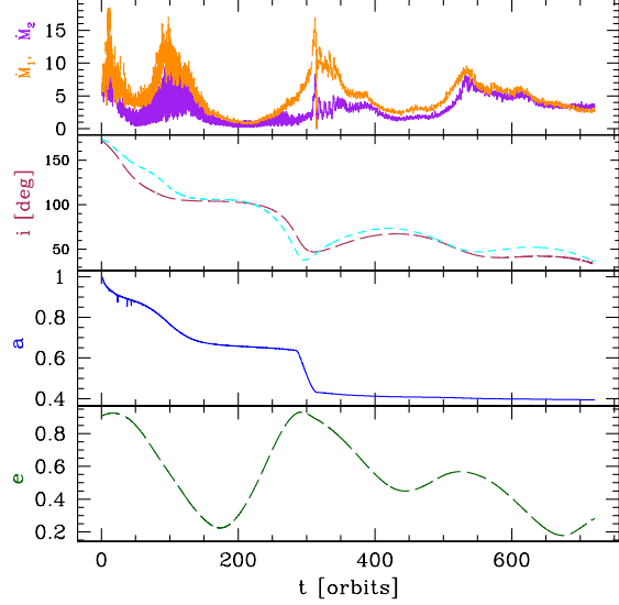
Figure 10. RETROGRADE HIGH ECCENTRICITY RUN, TILTING OF THE BHB - The retro** \epsilon = 0.9 run; from the top to the bottom, panels show the individual accretion rates \dot{M}_1, \dot{M}_2 ( \times 1000 ), the total inclination i in degrees, the inclination i_{2.5} towards only the inner rings , semi-major axis a and the eccentricity e . See text for more details; quantities are in code units.
