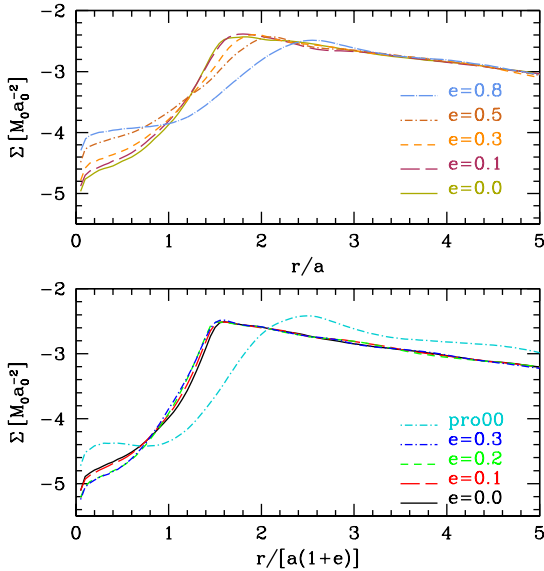
Figure 1. RETROGRADE RUNS, AVERAGE SURFACE DENSITY \Sigma(r) - Top : ”retro runs. Bottom : constant (1+\epsilon)a runs ”count” runs, Additionally, the circular prograde case is overlaid, in which the surface density peaks at a radius that is 1 a larger than in the retrograde case. Note that M_{\text{Disc}} in the count runs is smaller than in the retro runs. See text for more details; quantities are in code units.
