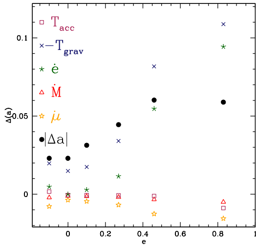
Figure 7. CONTRIBUTIONS TO \dot{a} BY INDIVIDUAL COMPONENTS; the pro00 run is inserted as negative e . Terms color-coded according to Eq. 3.
