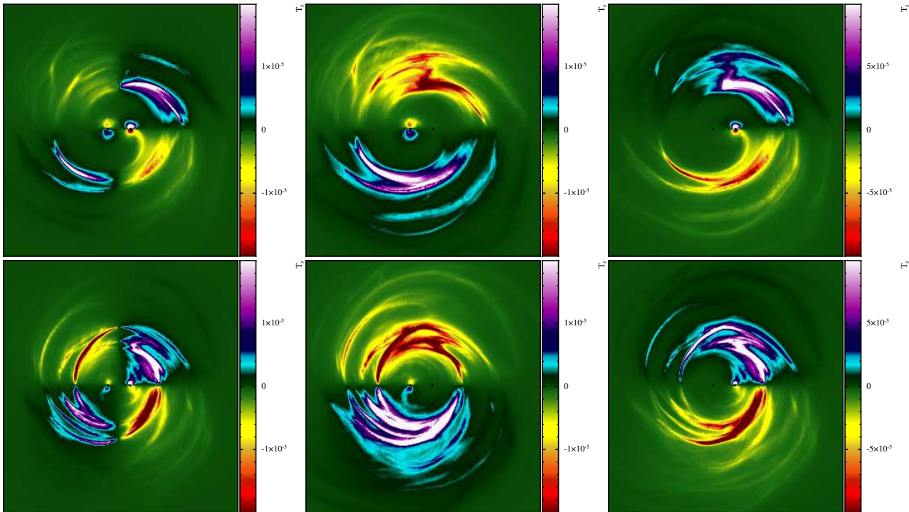
Figure 5. GRAVITATIONAL TORQUE DENSITY - Differential torque density in the z -direction for two initially circular BHB runs after 70 orbits. Top (bottom) panels: pro \epsilon = 0 (retro \epsilon = 0 ). In each row, from left to right we show the total torque density on the binary T_{G,z} = M_1 T_{G,z_1} + M_2 T_{G,z_2} , the torque onto the primary BH, T_{G,z_1} , and the torque onto the secondary BH, T_{G,z_2} . Figure made using SPLASH (Price 2007).
