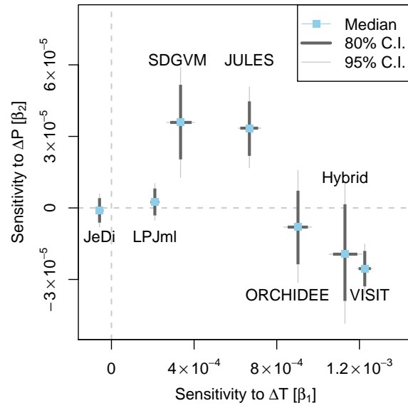
FIGURE S3. Sensitivity of global SOC stocks in response to \Delta T and \Delta P in each biome model
