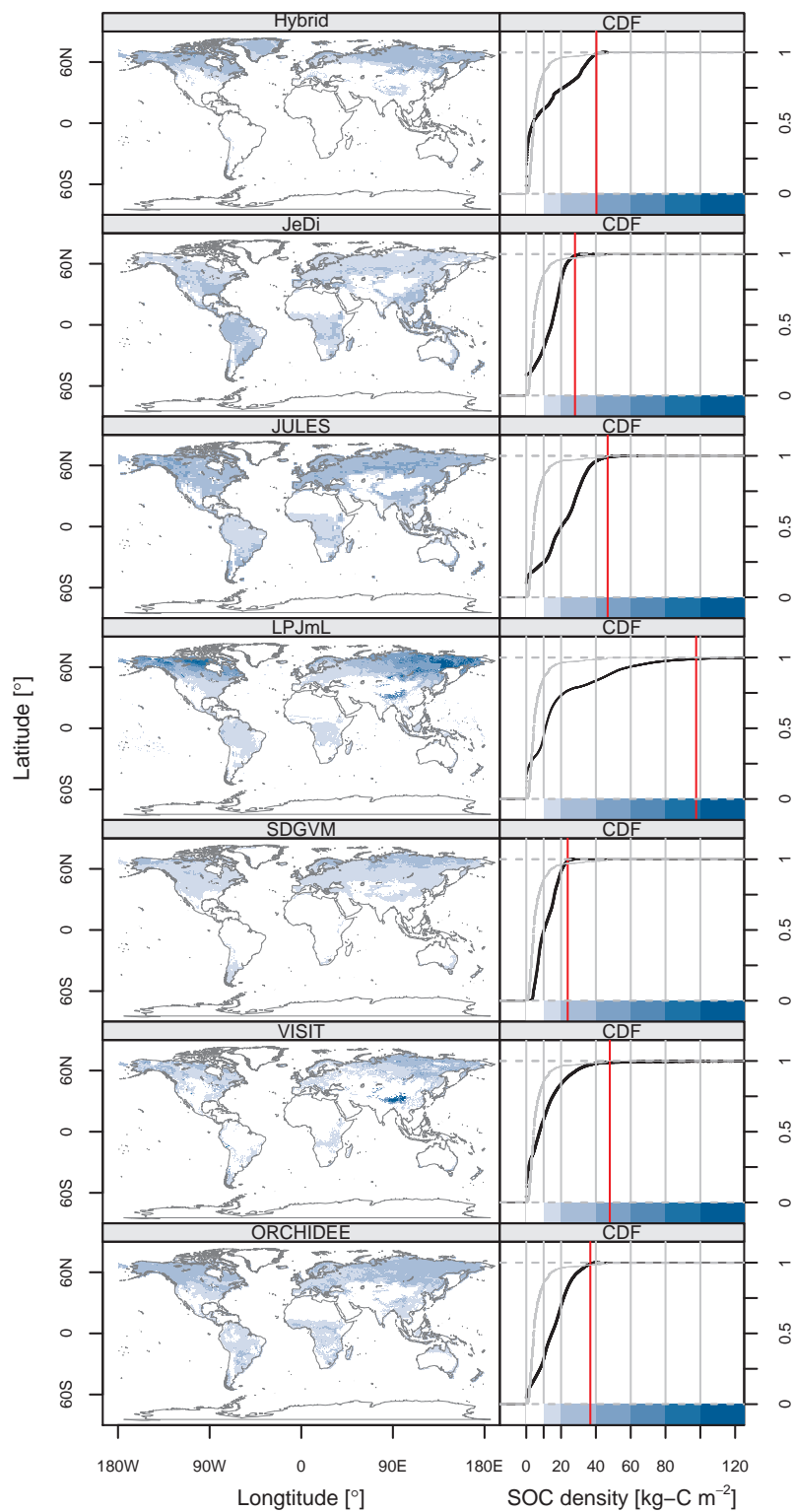
FIGURE S1. Maps of SOC density in 2000 and CDF in each biome model with HadGEM RCP8.5. In CDFs, red line indicates the 99th percentile of SOC density. In each CDF, grey lines indicate the CDF from the SOC density from the original Harmonized World Soil Database.
