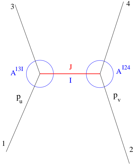
Fig. 4: At fixed impact parameter we find a contribution to the amplitude given by the on-shell propagator in the intermediate channel, labeled by the letter I . The contribution involves a product of two on-shell intermediate amplitudes, \mathcal{A}^{13I} and \mathcal{A}^{I24} , which are circled in the figure. Particles 1 and 3 carry a large momentum p_u and 2 and 4 have a large p_v . We get a factor of s^J from contracting p_u on the left side with p_v on the right side through the sum over polarizations of the intermediate particle.
