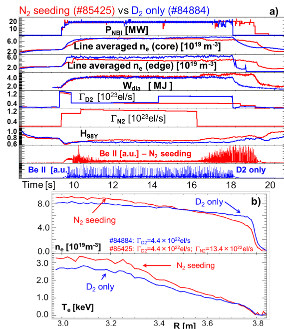
Fig.1 Comparison between nitrogen seeded plasma (red) and plasma pulse fuelled with D 2 only: time traces (a) and n e and T e profiles (b).
