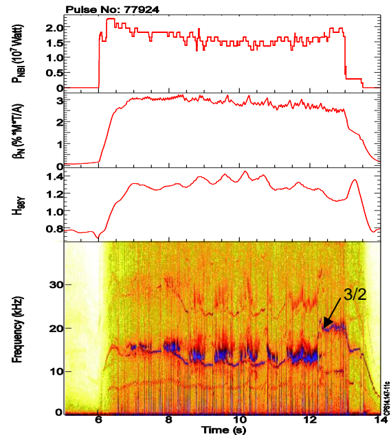
Fig 5 High performance hybrid C-wall pulses. The n =1 activity at ~15kHz has no significant effect on confinement. Later in both pulses a n >1 mode develops and the 3/2 mode does affect performance.
