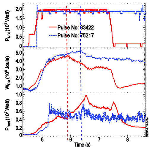
Fig 3 Comparison of 2 pulses with ILW (red) and C-Wall (blue). The vertical broken lines show the 3/2 NTM timing.
