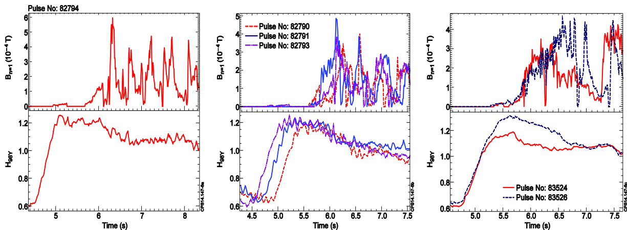
Fig 6 High performance hybrid ILW pulses in which only core n=1 activity occurs. In all cases n=1 activity degrades confinement. A range of pulses are shown to highlight that the degradation is a common event.
