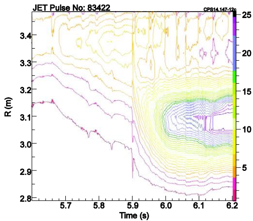
Fig 4 Vertical SXR camera – the radii (R(m)) are the intersection radii of the SXR chord with the midplane. The NTM at 5.9s causes the off-axis impurity localisation to rapidly peak on-axis.
