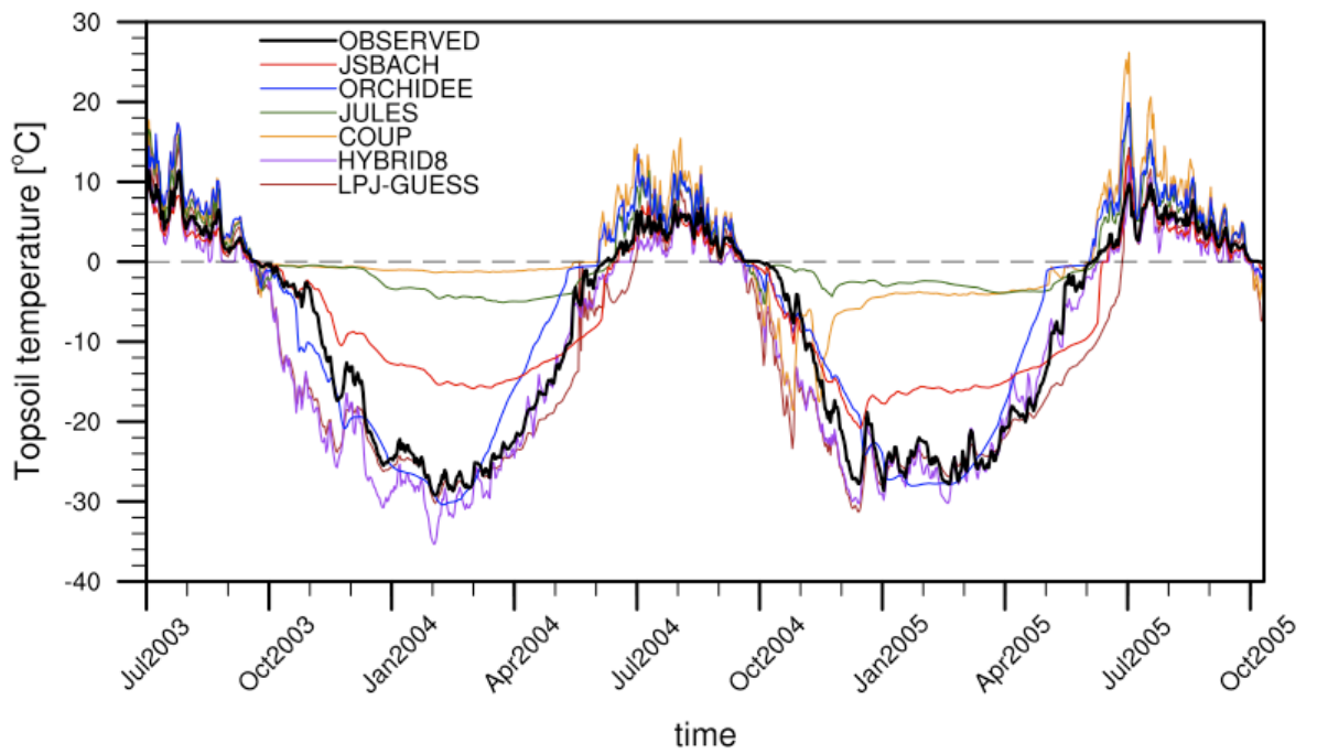
Figure 3: Timeseries of daily topsoil temperature from observations and models at the Samoylov site.
