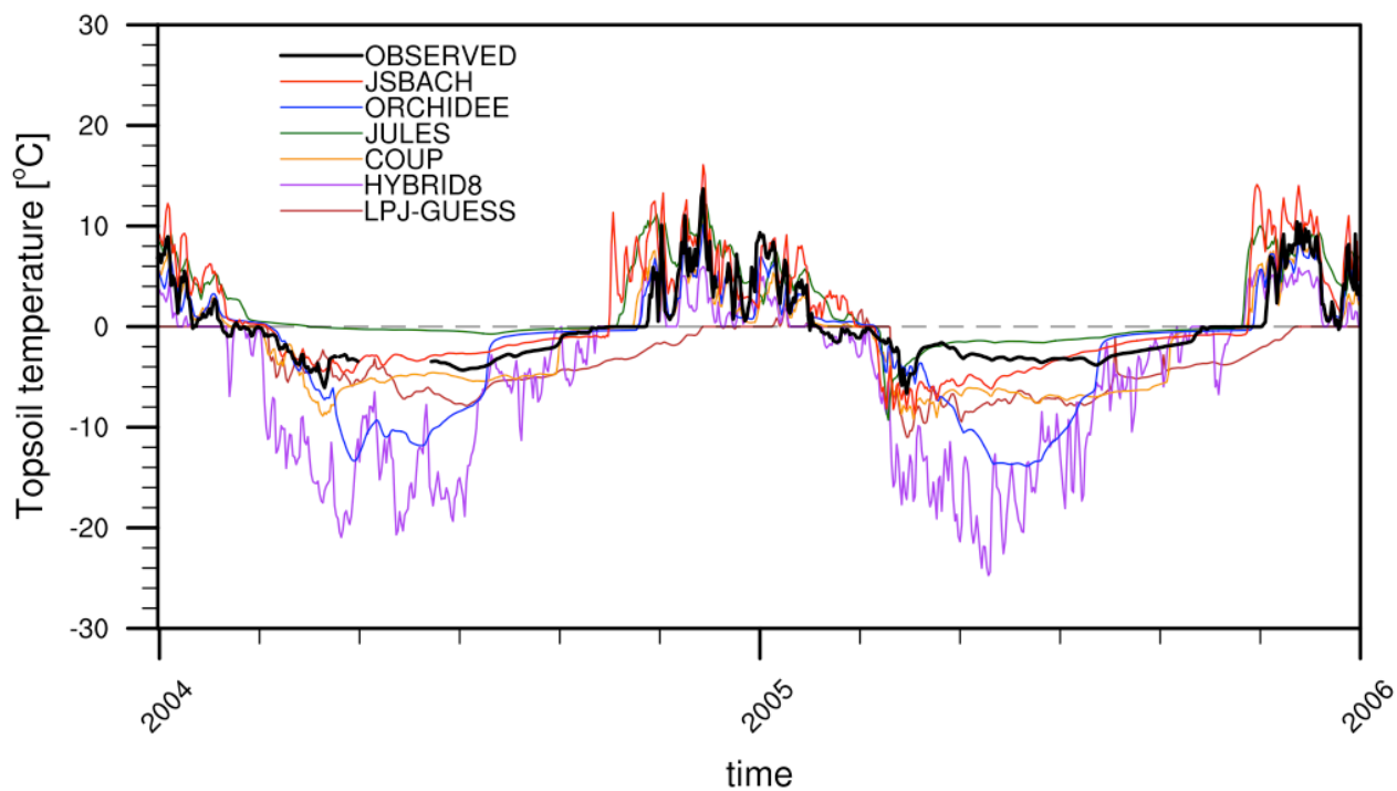
Figure 2: Timeseries of daily topsoil temperature from observations and models at the Schilthorn site.
