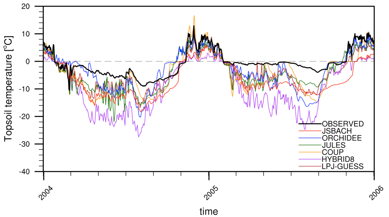
Figure 4: Timeseries of daily topsoil temperature from observations and models at the Bayelva site.
