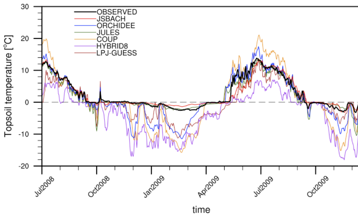
Figure 1: Timeseries of daily topsoil temperature from observations and models at the Nuuk site.
