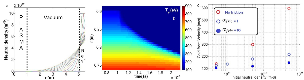
Figure 3: IMAGINE simulation results for a MGI of deuterium in JET: a. Successive neutral density profiles, b. Evolution of electron temperature, c. Influence of friction parameter and number of particles injected on the cold front velocity
