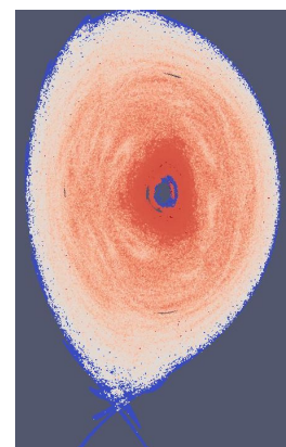
Figure 2: Poincaré plot during the TQ
