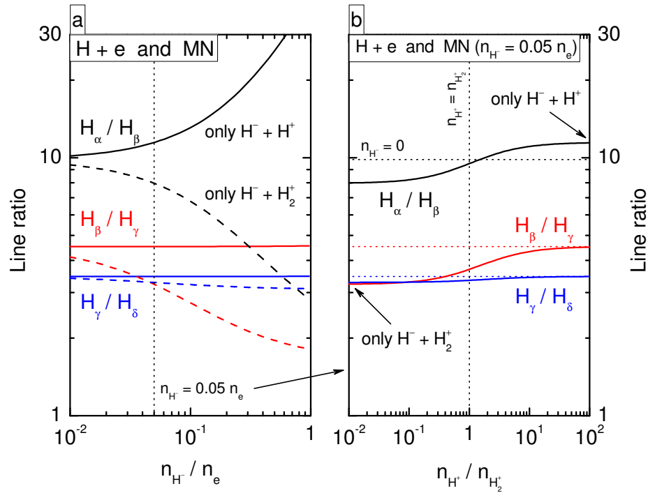
Figure 6.17: (a) Line ratios influenced by the mutual neutralization reactions (MN with H^+ : solid lines; MN with H_2^+ : dashed lines) with increasing ratio of the negative ion density to the electron density. T_e , n_e and n_H as in figure 6.16, n_{H^+} and n_{H_2^+} equal 0.4 n_e , respectively. (b) Influence of MN on the line ratios at varying positive ion composition for constant n_{H^-} = 0.05 n_e and n_{H^+} + n_{H_2^+} = 0.4 n_e .
