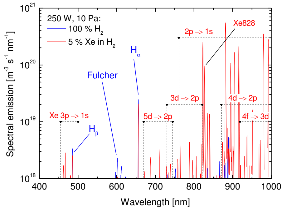
Figure 9.1: Exemplary spectra of the ICP discharge for a pure hydrogen plasma and with 5% admixture of xenon at an absolute pressure of 10 Pa and 250 W RF power. The dominant emission lines and systems are denoted.
