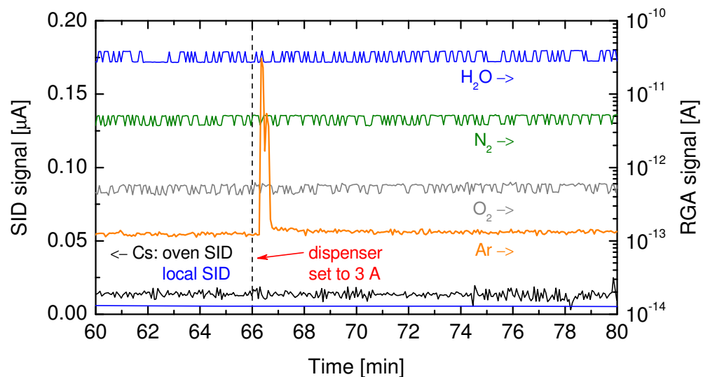
Figure 7.5: Demonstration of the activation procedure for Alvatec dispensers at 3 A dispenser current, monitored by signals from both SIDs (the blue curve at the bottom corresponds to the local SID) and pertinent RGA signals. The oven temperature is constant at 150 °C.
