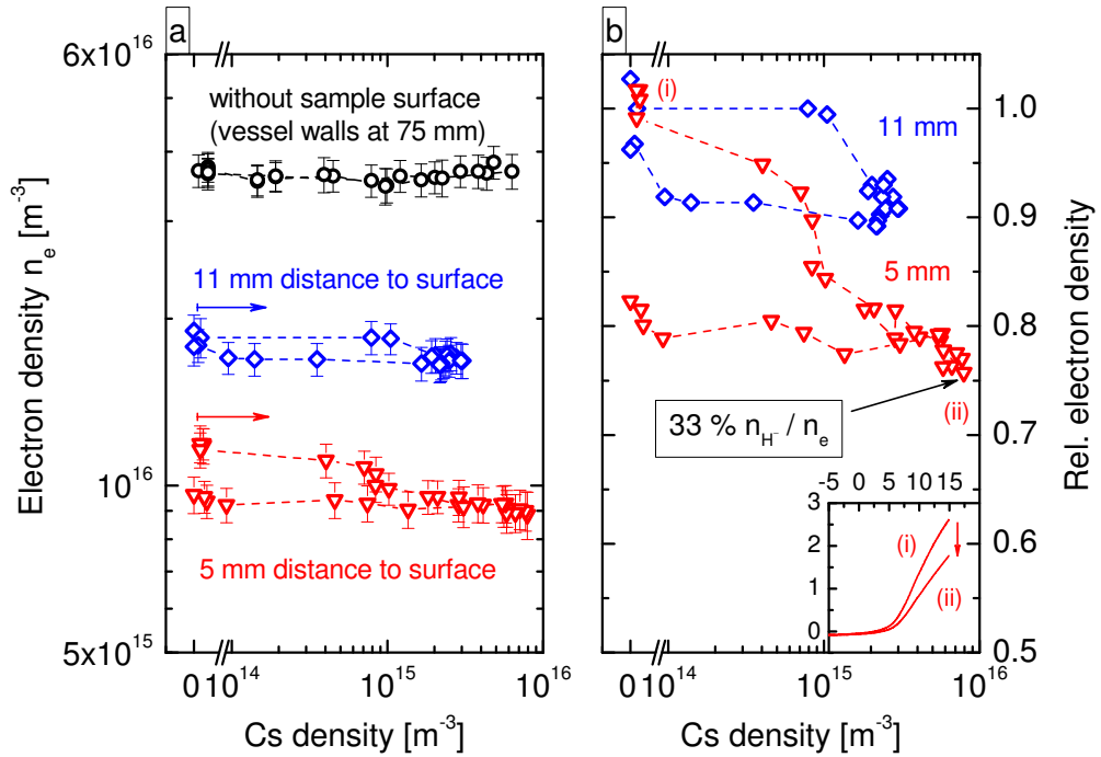
Figure 9.18: Electron density depending on the Cs density in a H_2 plasma at 10 Pa and 250 W for different distances from a stainless steel surface (see figure 9.16). (a) Absolute values. (b) Relative values. The arrows in (a) denote the beginning Cs evaporation and the inlet in (b) shows two exemplary I-V curves ( [mA]-[V] ) from the Langmuir probe at 5 mm distance for (i) infinitesimal and (ii) high Cs density.
