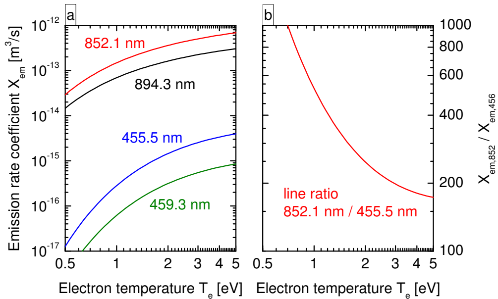
Figure 6.6: (a) Emission rate coefficients for the resonance lines of Cs, calculated after equation (6.18). (b) Line ratio of the Cs lines at 852.1 nm and 455.5 nm.
