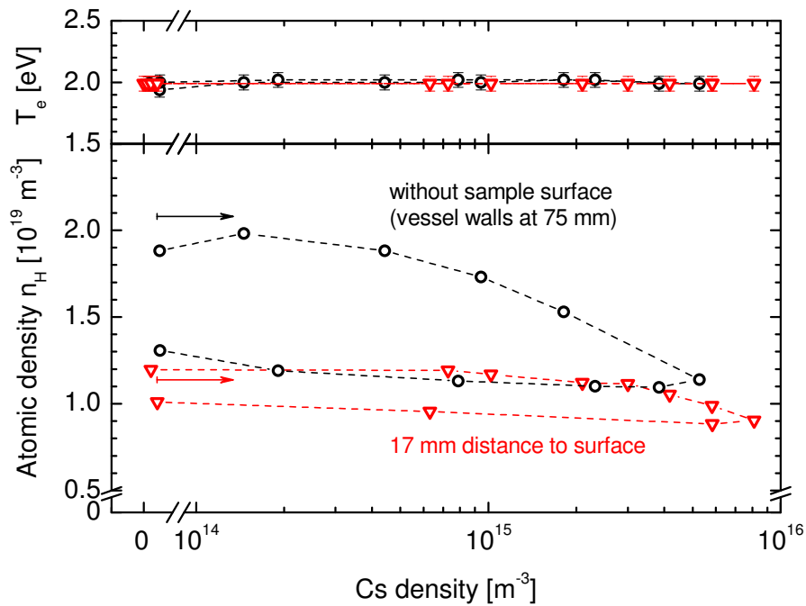
Figure 9.17: Electron temperature and atomic hydrogen density depending on the Cs density in a \text{H}_2 plasma at 10 Pa and 250 W for two different distances to the closest surface. The starting point of beginning Cs evaporation is denoted by arrows.
