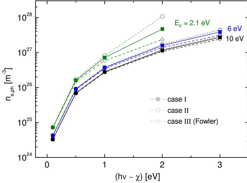
Figure 6.11: Density of photoelectrically releasable electrons calculated for different cases of approximation, each for three different Fermi energies and for T = 300\text{ K} .
