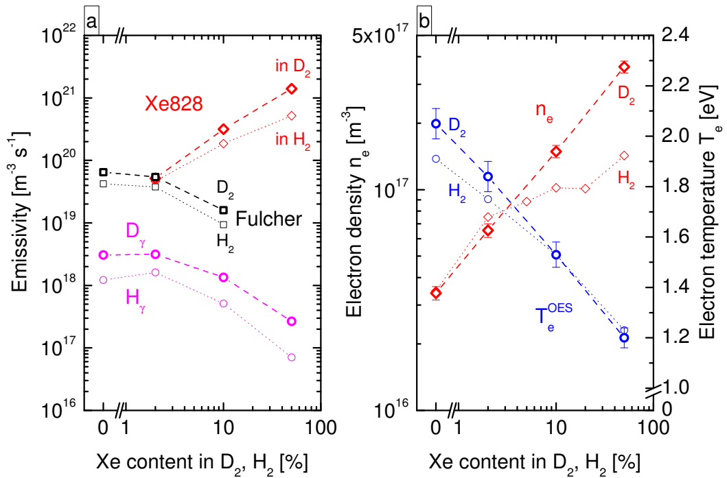
Figure 9.5: Influence of xenon admixtures to a deuterium plasma at 10 Pa absolute pressure and 250 W RF power on (a) the plasma emission and on (b) the electron temperature and density. Results for H 2 from figures 9.2 (a) and 9.3 (a) are plotted for comparison.
