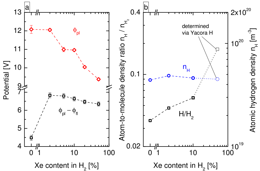
Figure 9.4: (a) Plasma potential and potential drop to a floating body in a plasma at 10 Pa absolute pressure and 250 W RF power with varying content of xenon in hydrogen. (b) Atom-to-molecule density ratio and atomic hydrogen density for the same parameters as in part (a).
