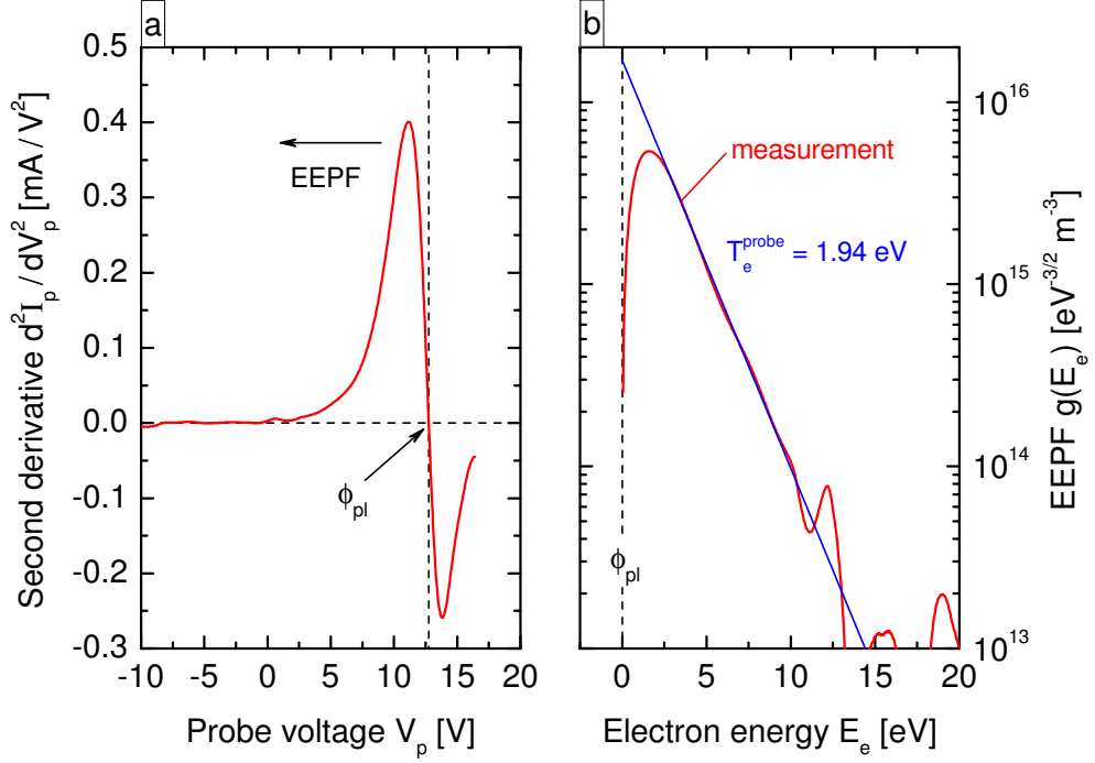
Figure 6.14: (a) Second derivative of the probe characteristic of figure 6.13 illustrating the determination of the plasma potential and the position of the EEPP. (b) Determination of T_{e,p} from a measured EEPP, which is calculated after equation (6.38).
