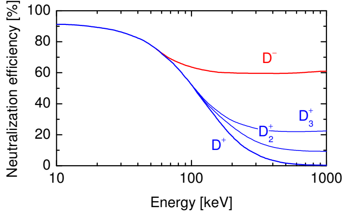
Figure 2.1: Neutralization efficiency of ion beams traveling through a D_2 gas target at rest with optimized thickness depending on the beam energy after [BPS75].
