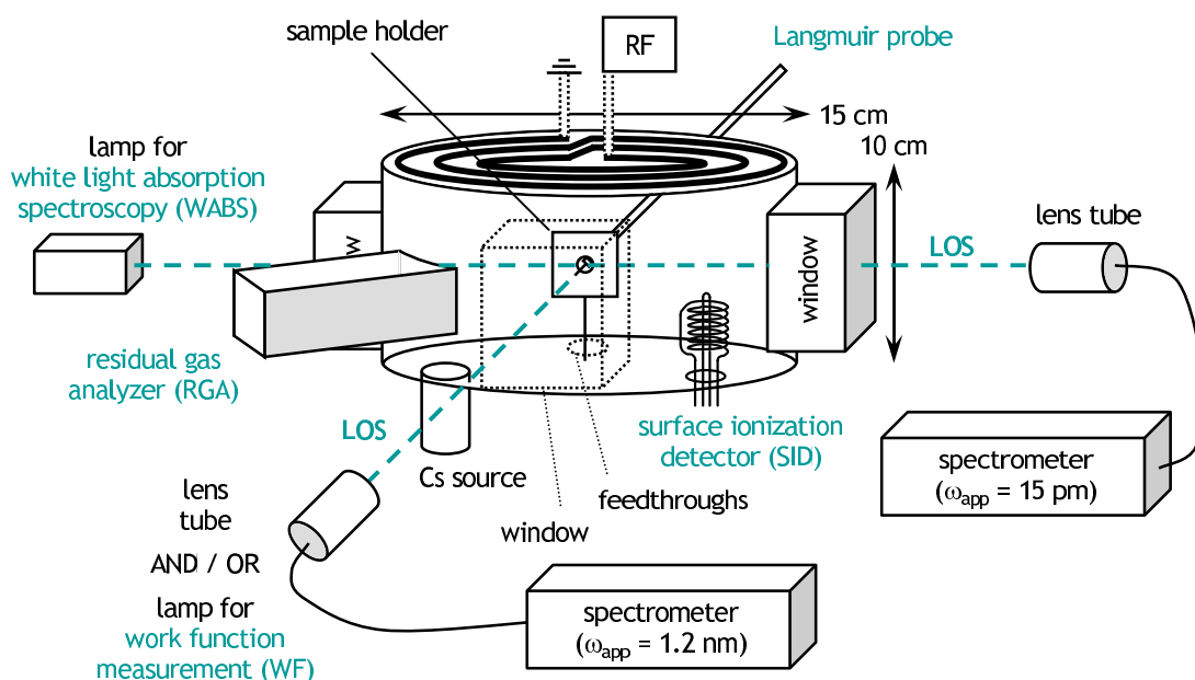
Figure 5.1: Perspective view of the schematic experimental setup with an overview of the arrangement of the equipment.
