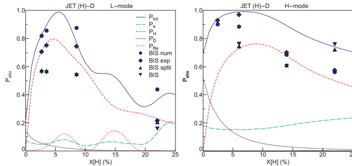
Figure 1: Heating efficiency in (a) L-mode and (b) H-mode as a function of the minority concentration. The symbols represent the experimental data inferred from BIS analysis; the lines are the corresponding theoretical predictions for the absorption in a full transit over the plasma.
