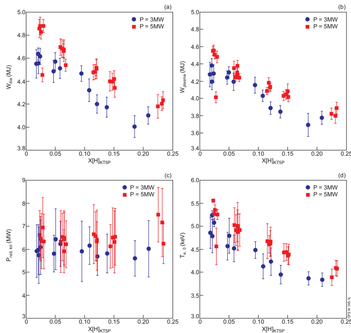
Figure 2: Diamagnetic energy (a), plasma stored energy (b), total radiated power, (c) and ECE central electron temperature (d) as a function of the minority concentration evaluated spectroscopically in the edge from the ratio of line intensities H_{\alpha}/D_{\alpha} (KT5P diagnostic).
