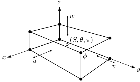
Figure 2: Sketch of a cell of the staggered grid. The prognostic variables are located at the cell centre ( \circ ), velocities are located at the cell faces ( \bullet \rightarrow ) and the level set scalar is located at the cell corners ( \bullet ).
