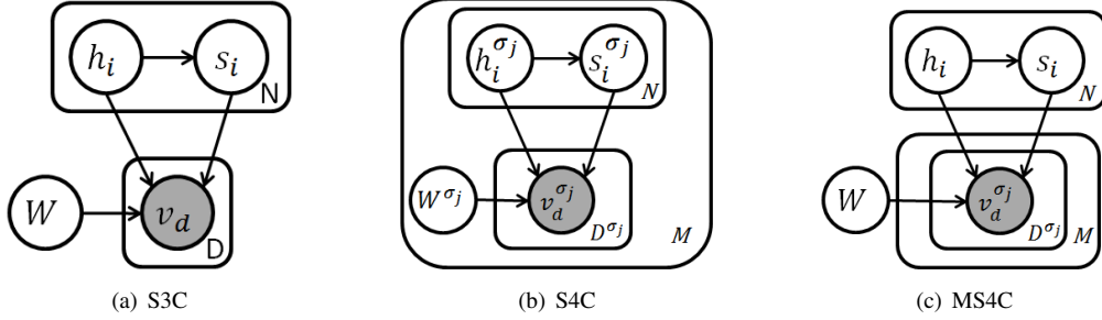
Figure 5. Multi-scale feature models. (a) S3C, (b) S4C, (c) MS4C.
