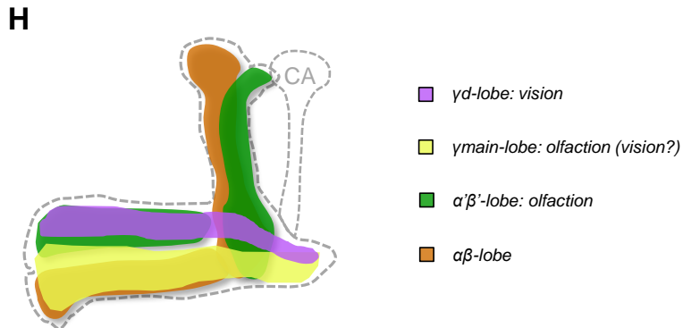
Figure 26: MB \gamma -lobes are required for visual but not aversive olfactory memory.
