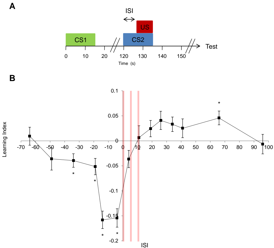
Figure 14: Timing dependent memory formation in Drosophila .
