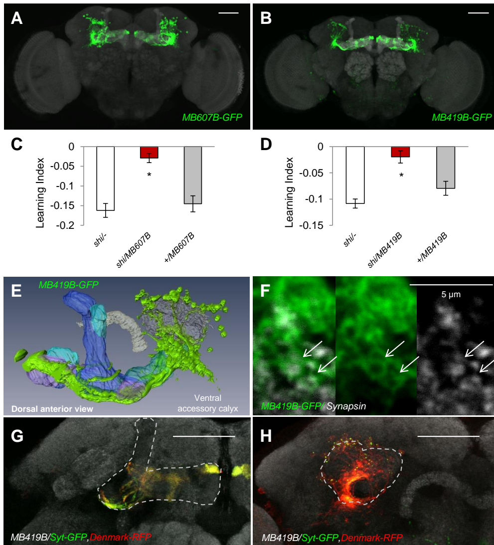
Figure 34: yd KCs possess a specific ventral accessory calyx (VACA).
