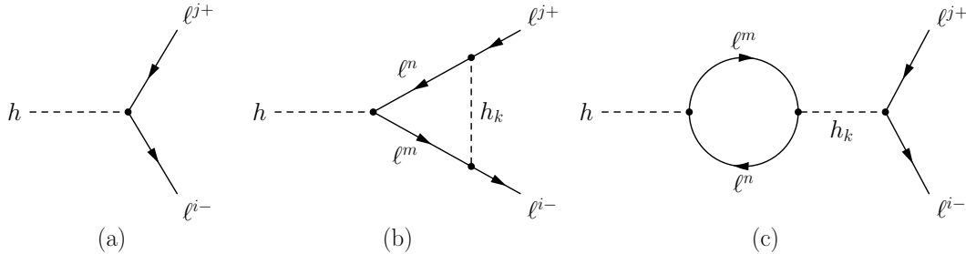
Figure 1: Feynman diagrams contributing to flavor and CP violating Higgs boson decays h \rightarrow \ell^{i-} \ell^{j+} . In the effective theory model (sec. 2.1), only one Higgs boson h \equiv h_1 exists and the bubble diagram (c) does not contribute to the CP asymmetry A_{CP}^{\ell^i \ell^j} . In the two Higgs doublet model (sec. 2.2, there are three physical neutral Higgs mass eigenstates h_1, h_2, h_3 , and all three diagrams contribute to A_{CP}^{\ell^i \ell^j} .
