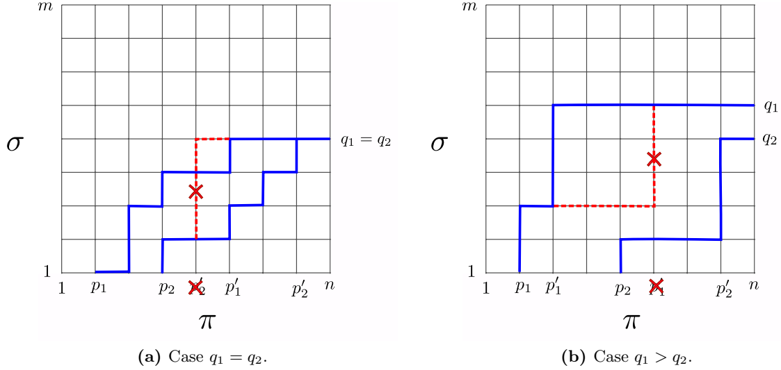
Figure 5: Illustration of Lemma 4.22. For both p_i, i \in \{1, 2\} , a feasible traversal of the curves \pi_{p_i..p'_i} and \sigma_{1..q_i} is depicted as monotone paths in the free-space.
