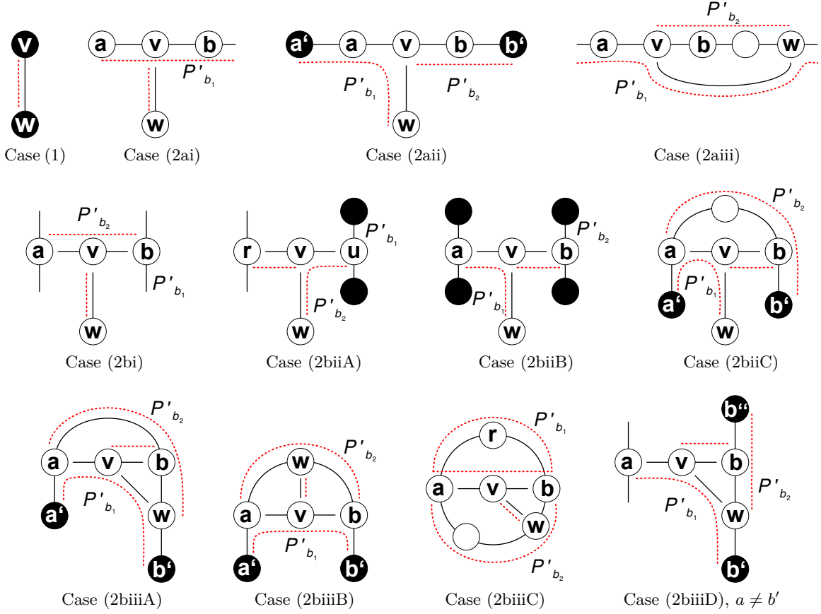
Figure 3: Cases (1) and (2) of Lemma 17. Black vertices are endpoints of ears that are contained in G_{birth(b)} . The dashed paths depict (parts of) the ears in D' .
