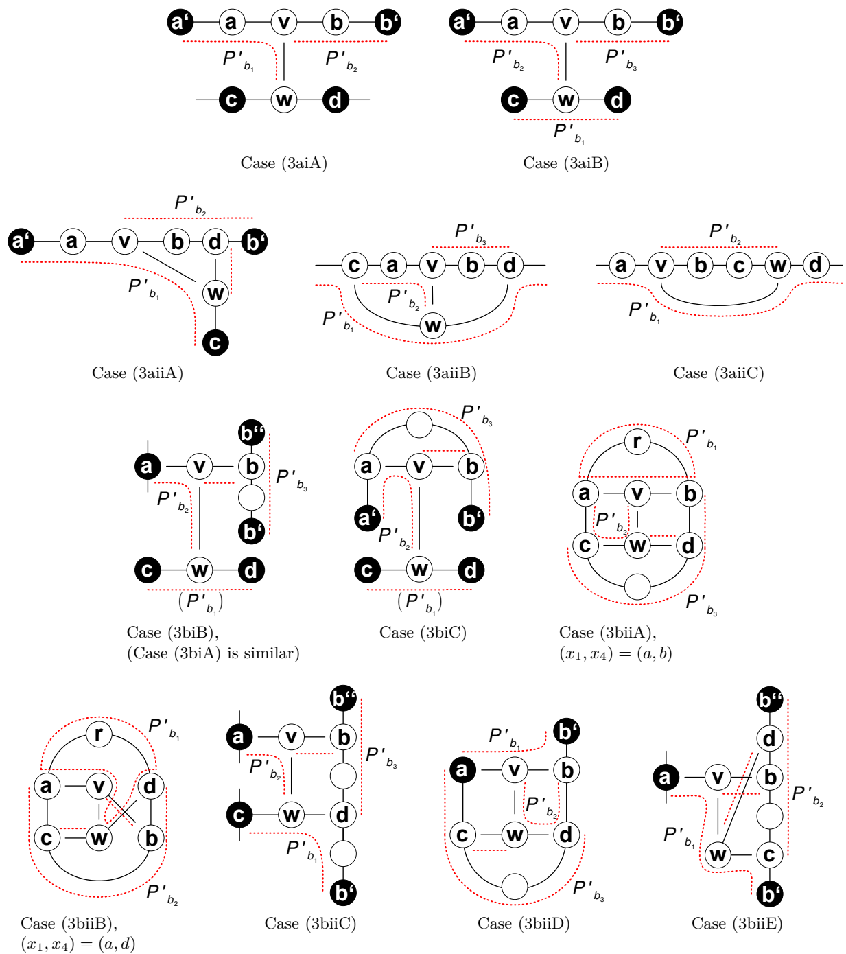
Figure 4: Case (3) of Lemma 17.
