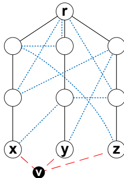
Figure 6: A spanning subgraph of a 3-connected graph G . G is obtained from the 3-connected graph G' := G - v \cup xy by a BG-operation (or inverse contraction) that adds the vertex v . Two of the three independent spanning trees of G' are given, rooted at r (solid and dotted edges). However, not both of them can be completed to cover v in G .
