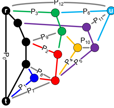
Figure 1: A Mondshein sequence of a non-planar 3-connected graph.
