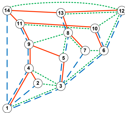
Figure 5: Three independent spanning trees in the graph of Figure 1, which were computed from its Mondshein Sequence (vertex numbers depict the consistent st-numbering).
