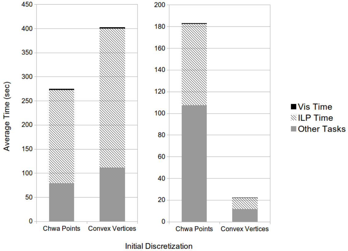
Figure 7: Average Time needed to solve ortho-ortho (left) and spike (right) polygons with 1000 vertices using the Convex Vertices and the Chwa Points discretization.
