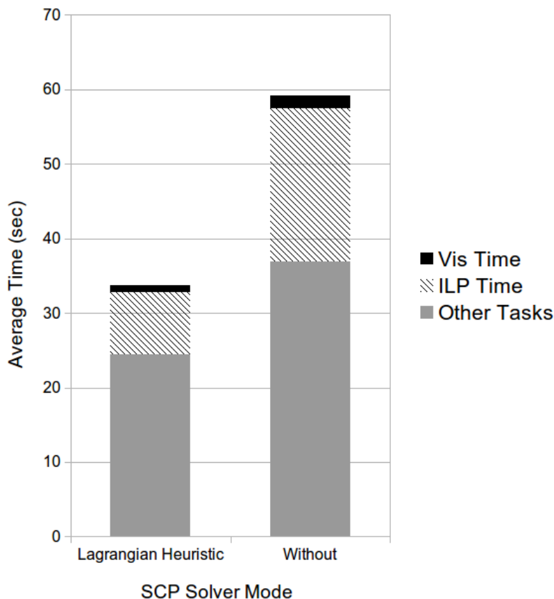
Figure 5: Average Time needed for the current Campinas version to solve von Koch polygons with 1000 vertices with and without the Lagrangian Heuristic.
