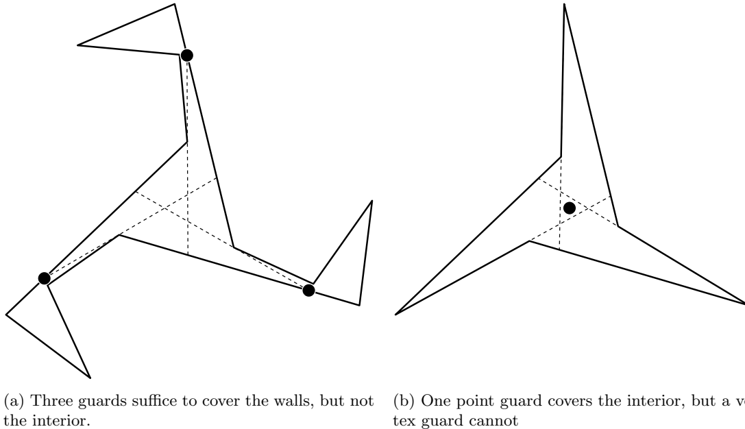
Figure 1: Edge cover and vertex guard variants have better and worse solutions than the classic AGP, respectively.
