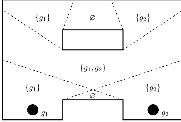
Figure 2: The visibility arrangement \mathcal{A}(\{g_1, g_2\}) induced by two guards g_1 and g_2 in a polygon with one hole.
