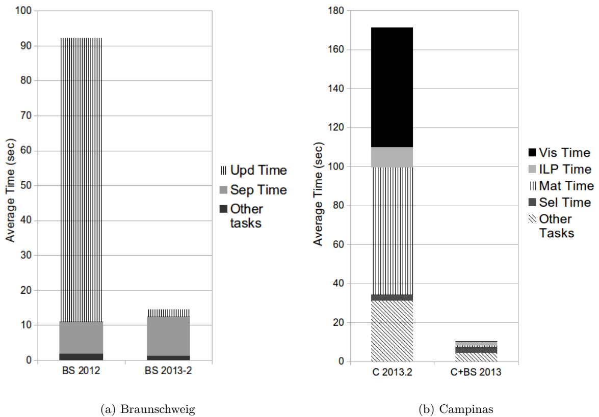
Figure 4: Split up of average total time for different configurations on all simple instances with 1000 vertices. (left) The update time which is dominated by the visibility polygon computation almost vanishes in BS-2013 compared to the BS-2012. (right) The time spent on visibility in C+BS-2013 is almost negligible compared to the time spend in C-2013.2.
