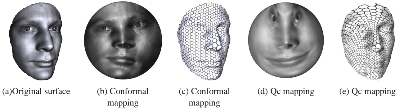
Figure 1: Conformal and quasiconformal mappings from a human face surface to the planar disk.
