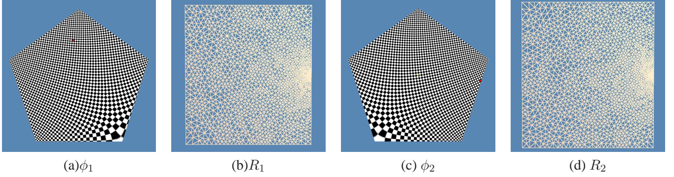
Figure 3: Holomorphic quadratic differential bases on a pentagon.
