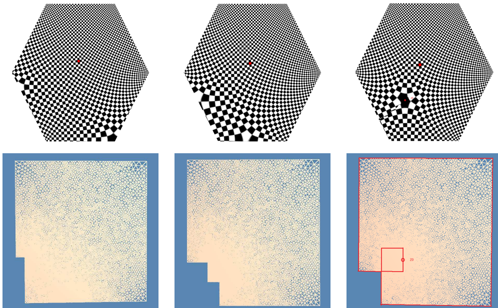
Figure 6: Holomorphic quadratic differentials on a hexagon.
