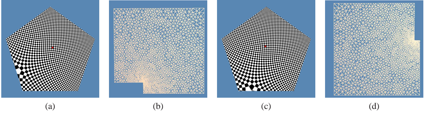
Figure 4: Holomorphic quadratic differentials on a pentagon. (a) and (b) show [0.2(\phi'_1)^2 + 0.8(\phi'_2)^2]dz^2 , (c) and (d) show [-0.2(\phi'_1)^2 + 1.2(\phi'_2)^2]dz^2 .
