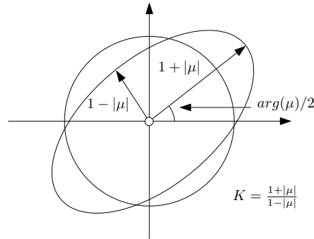
Figure 2: Beltrami coefficient.
