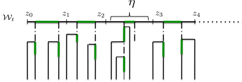
Figure 1: The first application of Lemma 4.4 gives a family of disjoint walks intersecting \mathcal{W}_t denoted by -\cdot- . Bold and green lines indicate the intersection of two walks. Second application of the lemma with the validity property gives the second level of disjoint walks.
