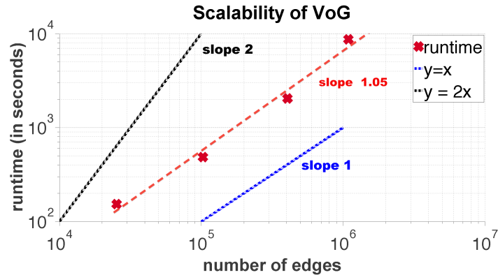
Figure 5: VOG is near-linear on the number of edges. Runtime, in seconds, of VOG (PLAIN) vs. number of edges in graph. For reference we show the linear and quadratic slopes.
