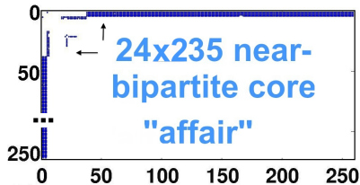
Figure 4: Enron: Adjacency matrix of the top nb core found by VOG, corresponding to email communication about an “affair”.
