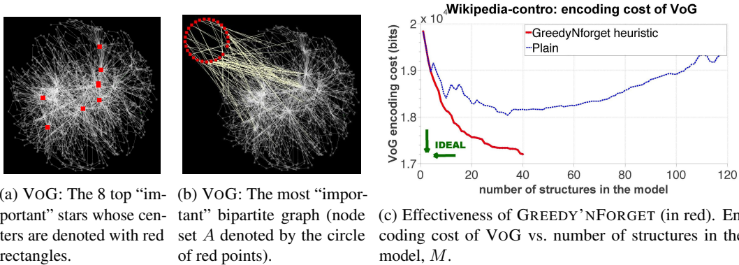
Figure 3: The VOG summary of the Controversy graph, and effectiveness of the GREEDY'NFORGET heuristic. The top 10 structures of the graph summary of VOG consist of 8 stars (Fig. 3a) and 2 bipartite graphs (Fig. 3b, 1d). Fig. 3c shows the encoding cost for the PLAIN (dotted blue line) and GREEDY'NFORGET (solid red line) heuristics. GREEDY'NFORGET minimizes the encoding cost by greedily selecting from a sorted, in decreasing quality order, set of structures the ones that reduce the cost. Thus, GREEDY'NFORGET leads to better encoding costs and smaller summaries (here only 40 are chosen) than PLAIN ( \sim 120 structures).
