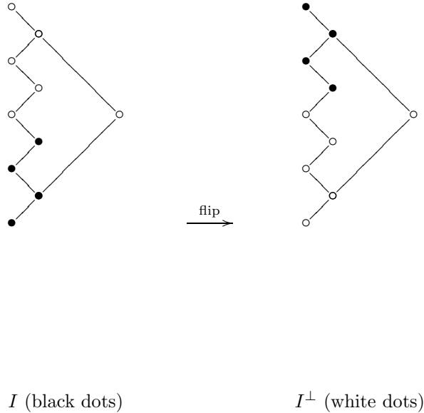
FIGURE 2. The involution on order ideals.
