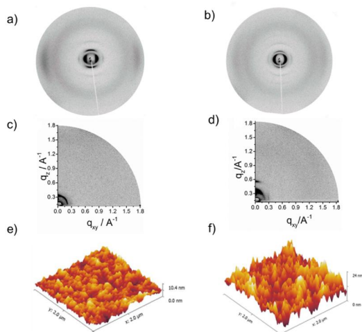
Figure 5. 2DWAXS patterns for extruded fibers of a) PBDTTQ-3 and b) PAPhTQ . The fiber sample was mounted vertically towards the detector. GIWAXS patterns for c) PBDTTQ-3 and d) PAPhTQ thin films. SFM topography images of PBDTTQ-3 (e) and PAPhTQ (f) thin film in the transistor channel. The RMS roughness values are 1.3 nm for PBDTTQ-3 film and 3.3 nm for PAPhTQ film, respectively.
