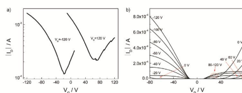
Figure 4. The transfer (a) and output (b) curves of PBDTTQ-3.
