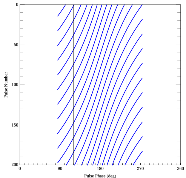
Figure 6. Curved subpulse driftbands of PSR B0818-42 generated through the SCLF model (solid blue lines), to be compared with those reported in Fig. 2 of Bhattacharyya et al. (2007). Tracks are plotted for the whole longitude range of the average profile, while vertical black lines indicate the boundaries of the region where drifting subpulses are actually observed.
