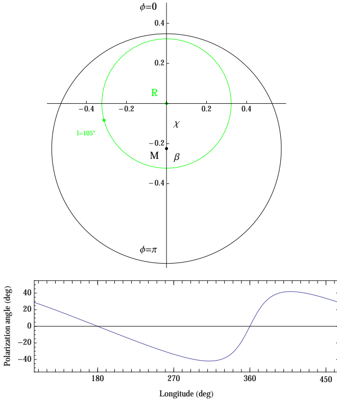
Figure 2. Upper panel: observing geometry of PSR B0826-34 (the coordinate axes show the values of the angular coordinate \theta in degrees). The black circle indicates the polar cap, with the center in the magnetic pole (black point "M"), while the green circle indicates the trajectory of the line of sight of the observer, with the center on the axis of rotation (green point "R"). " l = 105^\circ " (rather than l = 0^\circ ) is used as origin of the pulse longitude in order to bring the plots in the visual correspondence with the ones from the literature. Lower panel: Polarization angle as a function of longitude in our model. The plot is shifted in longitude for easier comparison with previous results from the literature (see discussion in the text).
