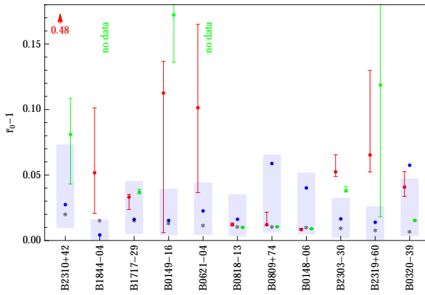
Figure 1. Values of the altitude above the surface of the star \bar{r}_0 - 1 obtained by solving the equation (14) for the pulsars of Table 1. Red points correspond to the observing wavelength at 21 cm, green points correspond to the observing wavelength at 92 cm. The obtained altitudes are compared to the PFF from Hibschan & Arons (2001) (blue shadowed regions) and Harding & Muslimov (2001, 2002) (blue points). Black stars show the angular radius of the polar cap \Theta_0 . Special cases are indicated as described in the text. The figure does not report the two sources B1702-19 and B2045-16. The first one does not admit a solution of Eq. (14) for any radial coordinate, while the second one has opposite sense of the subpulse drift for the observations at 21 cm and 92 cm.
