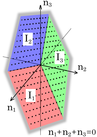
FIG. 1. Admissible instanton numbers for various complex structures on \mathcal{F}_3 are shown by black dots.
