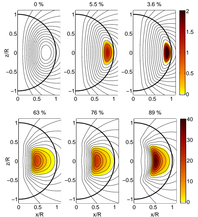
Fig. 2 Top panels: Meridional view of twisted-torus magnetic field configurations obtained with the simple commonly-adopted current prescription (see Ciolfi & Rezzolla 2013 for details). Shown in colour is the toroidal-field strength in units of the polar value. R is the stellar radius. The labels on top of each panel show the toroidal-field energy content relative to the total internal magnetic energy ( E_{\text{tor}}/E_{\text{m}}^{\text{int}} ). Bottom panels: The same as above for example configurations obtained with the novel prescription (cf. Section 2 of Ciolfi & Rezzolla 2013).
