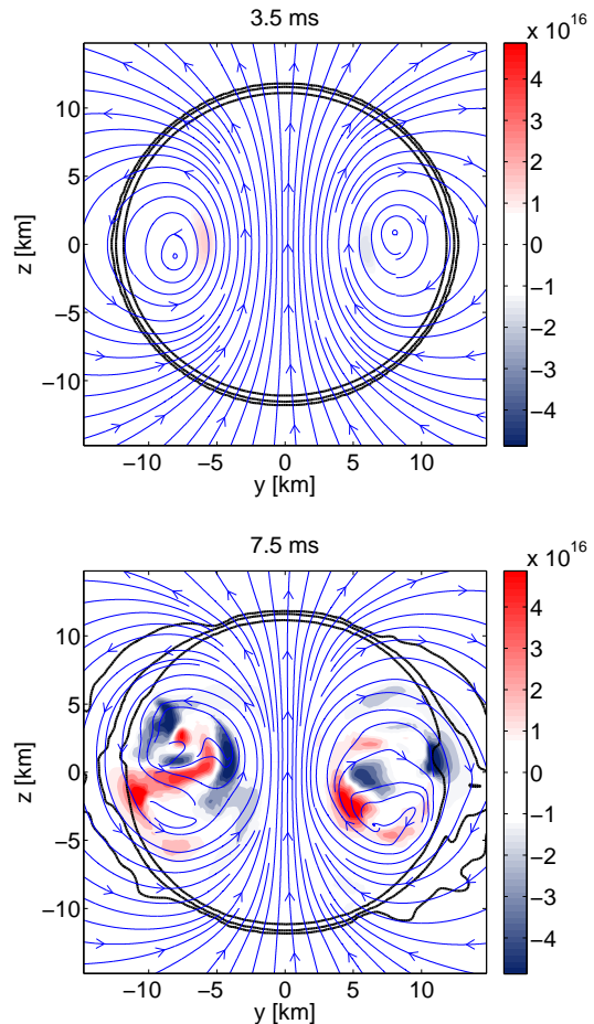
Fig. 1 Meridional view of the instability of a purely poloidal field in a magnetized NS with an initial polar magnetic field strength of 6.5 \times 10^{16} G. Poloidal field lines are shown together with the color-coded toroidal magnetic field strength; also reported are three rest-mass isodensity contours near the stellar surface, corresponding to (0.02, 0.2, 2) \times 10^{13} \text{ g/cm}^3 . The two frames illustrate respectively the saturation of the instability, which sets the beginning of the non-linear evolution, and the most violent phase of the field rearrangement, when the instability has fully developed. In this case the Alfvén timescale is \sim 3 ms.
