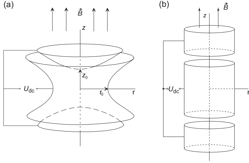
Figure 2.1: Schematic of (a) a hyperbolic and (b) a cylindrical Penning trap. The trapping potential is created by applying a voltage U_{\text{dc}} between the ring electrode and the endcaps. Radial confinement of the ion is achieved due to the superimposed homogeneous magnetic field in z -direction. The minimum distances from the trap center are indicated by z_0 in axial direction and r_0 in radial direction. Taken from [2].
