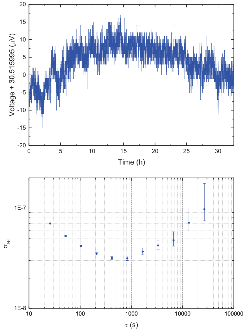
Figure 7.9: A Rev.0 channel in the precision mode at -30\text{V} was tested in the PENTATRAP laboratory at MPIK. The voltage data (top) are shown and the relative Allan deviation, i. e. the relative voltage stability (bottom) of \leq 4 \cdot 10^{-8} has been obtained for time intervals of about 10 minutes.
