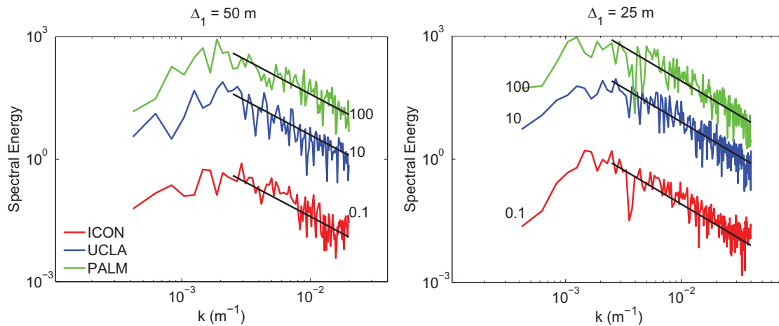
Figure 13. The horizontal spectra of the vertical velocity at indicated resolutions in log-log scale. The data have been multiplied by some factors in order to avoid overlap. Also shown is the expected Kolmogorov's spectrum ( \propto k^{-5/3} ) (black line), for \Delta_1 = 50, 25 m.
