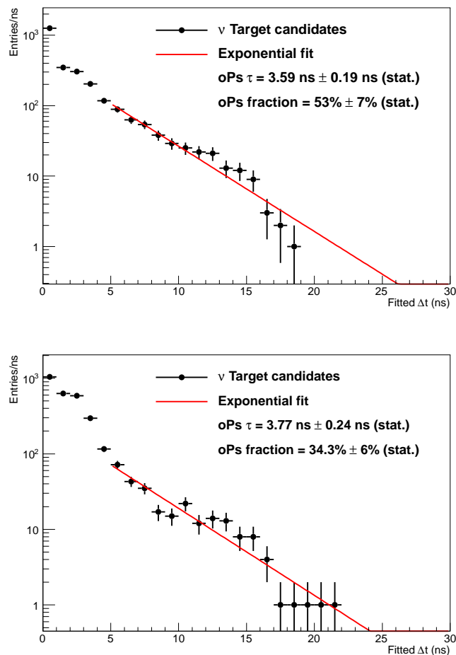
Figure 6: Fit of the \Delta t distribution, for neutrino candidates with energy between 1.2 and 3 MeV, with an exponential function for \Delta t greater than 5 ns. The 60 Co (top) and the 137 Cs (bottom) reference time profiles are used in the oPs tagging algorithm. The errors quoted on the figures are statistical only.
