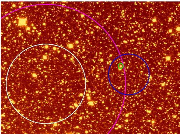
Fig. 1. 2MASS J19435624+2118233 and the VLBI, Chandra CXOU J194356.2+211823, HESS J1943+213, and Fermi objects. The 2MASS J19435624+2118233 VLBI and Chandra objects lie within the green circle. The blue circle denotes the error ( 1\sigma ) circle of the HESS observation, the white circle is the ( 1\sigma ) statistical error circle of the Fermi -LAT observation, and the pink circle marks the ( 2\sigma ) circle of the Fermi -LAT observation.
