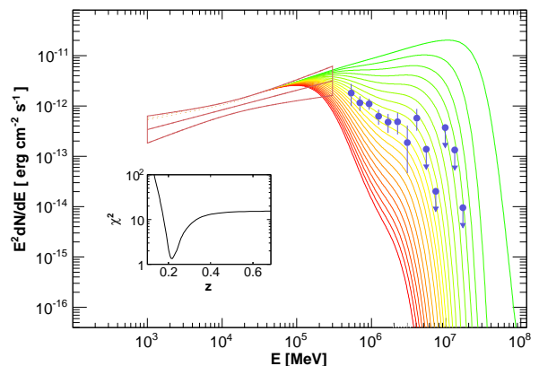
Fig. 6. Spectral energy distribution of HESS J1943+213 in \gamma -rays. The Fermi -LAT error contour (red) has been extrapolated towards the H.E.S.S. energy range (blue points) and corrected for EBL absorption using the model of Franceschini et al. (2008) assuming different values for z from z = 0.01 (green line) to z = 0.7 (red line). The inset gives the corresponding \chi^2 as a function of the redshift z .
