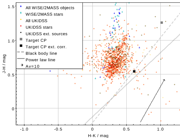
Fig. 2. Color-color plot in the J, H and K bands for the infrared sources within the error circle of HESS J1943+213. The infrared counterpart 2MASS J19435624+2118233 is clearly redder than the main distribution of sources in this direction of the sky. The arrow indicates the direction of reddening by extinction by interstellar dust for A_V = 10 .
