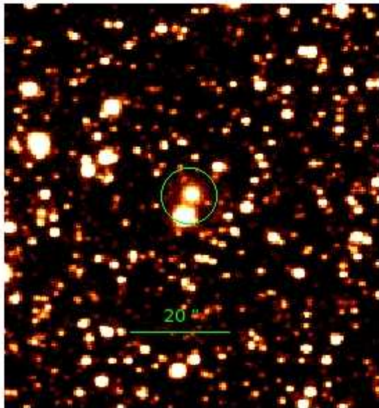
Fig. 4. The object and its neighbourhood is shown. The green circle is centered on the target. The object in the lower part of the circle is one of the stars ( \alpha_{J2000} = 19^{\text{h}} 44^{\text{m}} 00.0^{\text{s}} , \delta_{J2000} = 21^{\circ} 17' 16.1'' ) used to determine the target coordinates.
