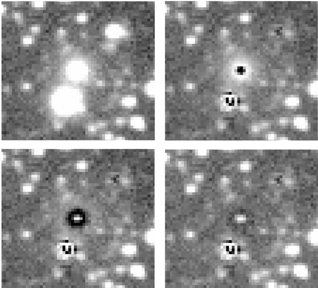
Fig. 5. K-band image of the infrared counterpart of HESS J1943+213 ( 25'' \times 25'' ). The image at the top left is centered on 2MASS J19435624+2118233 the prospective infrared counterpart of the VHE gamma-ray source. The next 3 panels show residuals after subtracting, at the top right , a point source, at the bottom row from left to right, an exponential surface brightness profile, and a surface brightness profile with Sérsic index 7. The package galfit was used to determine the best-fitting free parameters (magnitude and, for the extended profiles, half-light radius). Bright, neighboring stars were also subtracted to avoid confusion. The prominent residual after subtracting a point source clearly demonstrates that the infrared counterpart to HESS J1943+213 is extended (to be compared with the residual from the bright star directly below HESS J1943+213). Furthermore, a high-Sérsic index profile leaves a smaller residual than an exponential profile, indicating that the surface brightness profile of HESS J1943+213 follows that of a typical, massive elliptical galaxy more closely than that of a disk galaxy. The moderate residual for the high-Sérsic index model hints at the presence of a central point source, but imaging with higher resolution is needed to confirm this.
