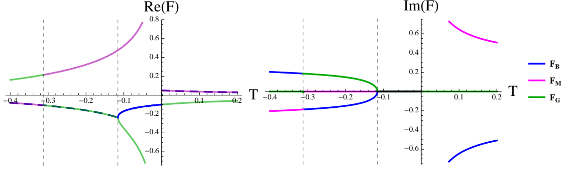
Figure 10. The solutions to the cubic for F as a function of T for \phi = 0.1, X = 0.1 .
