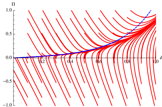
Figure 4. Trajectories in (\Pi, \phi) phase space for P_{FI}(X, \phi) with V_0 = 10 and T = 0.0001 .
