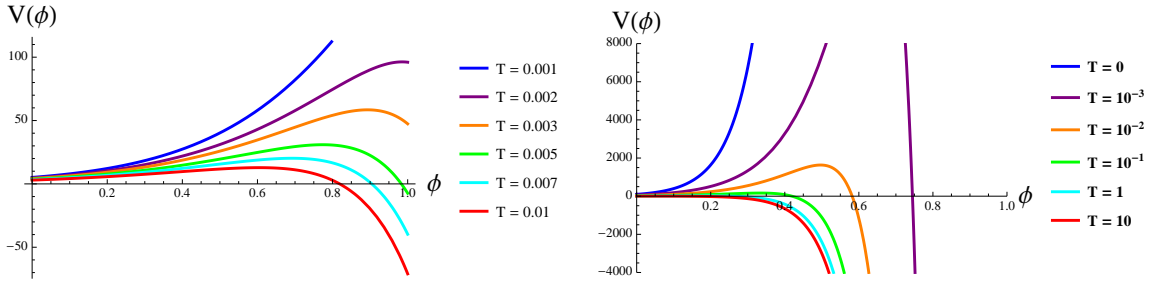
Figure 7. Effect of increasing T > 0 for an originally flat potential -P_{Fl}(0, \phi) for V_0 = 0.1 (left) and for an unstable potential -P_{Lin}(0, \phi) for c = 10 (right).
