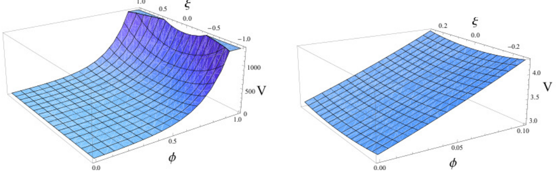
Figure 13. \xi potential from P_{CanK} for T = 0 (left) and T = 0.01 (right), with c = 3 .
