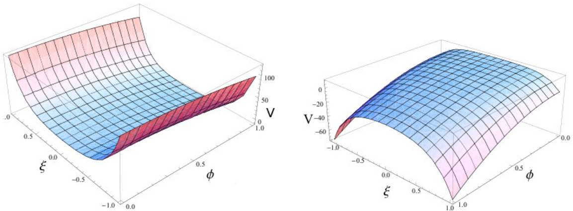
Figure 16. \xi potential from P_{Lin} for T = 0 (left) and T = 0.01 (right), with c = 3 . Note that the potential becomes negative when T is switched on, with c left the same.
