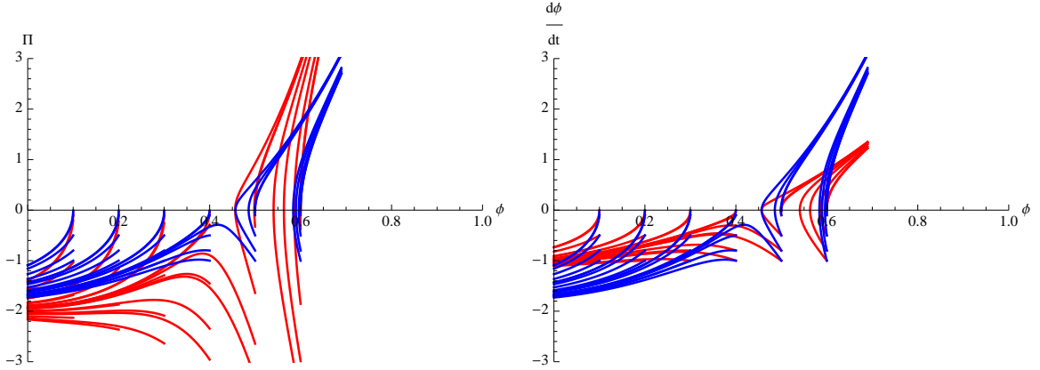
Figure 5. Trajectories in (\Pi, \phi) (left) and (\dot{\phi}, \phi) (right) phase space for P_{QuadK}(X, \phi) with c = 3 and T = 0.01 . The same trajectories for P_{QuadK}(X, \phi) with non-canonical kinetic terms switched off are in blue.
