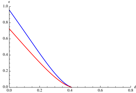
Figure 6. \epsilon(\phi) for P_{QuadK}(X, \phi) with c = 3 and T = 0.01 for a single trajectory. The same trajectories for P_{QuadK}(X, \phi) with non-canonical kinetic terms switched off are in blue.
