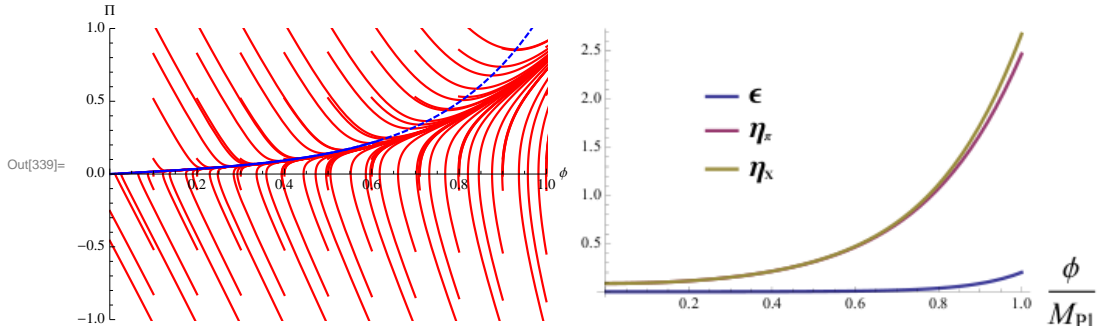
Figure 2. The blue line indicates the inflationary attractor (3.7) for P_{Fl}(X, \phi) with V_0 = 10, T = 10^{-3} (left). The line is solid until \eta_X and \eta_\Pi become greater than 0.5, and dashed from then on. The figure on the right shows the behavior of the generalized slow-roll parameters, evaluated along the blue solid/dashed line (3.7).
