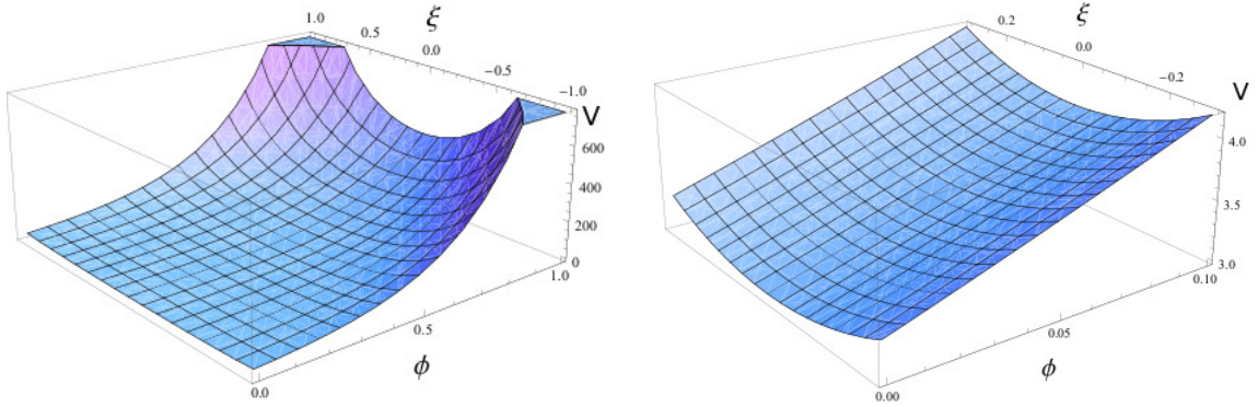
Figure 14. \xi potential from P_{QuadK} for T = 0 (left) and T = 0.01 (right), with c = 3 .
