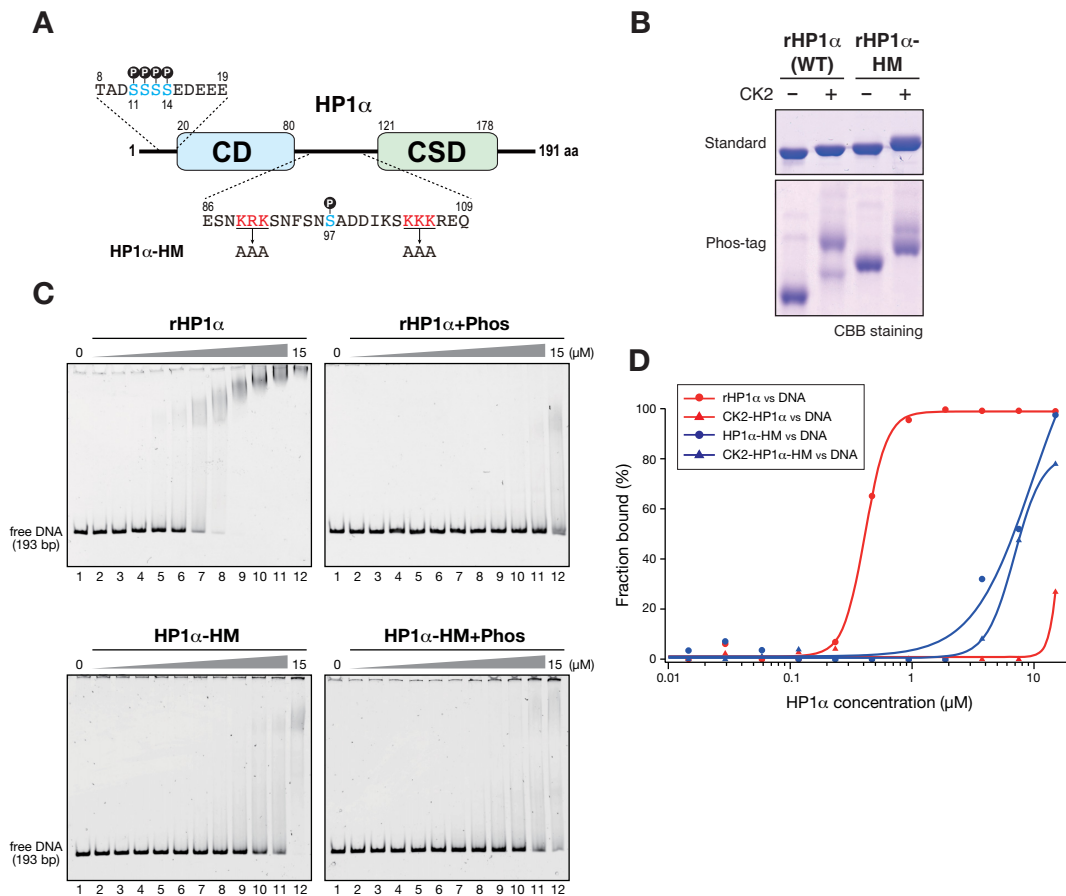
Figure 4. HP1 \alpha 's N-terminal phosphorylation inhibits its hinge region-mediated DNA binding. (A) Schematic diagram of HP1 \alpha showing amino acid sequences of the N-terminal and hinge regions, and the positions of amino acid substitutions in an HP1 \alpha with a hinge mutation (HP1 \alpha -HM). Phosphorylatable serine residues are shown in blue, and the basic residues replaced by alanine in the HP1 \alpha -HM are shown in red. (B) Control and CK2-phosphorylated WT and hinge-mutated (HM) HP1 \alpha proteins were resolved by standard or Phos-tag PAGE and visualized by CBB staining. (C) Representative EMSAs using control and CK2-phosphorylated WT and HM HP1 \alpha . The HP1 concentration varied from 0 to 15 \mu M (0.5-fold dilutions). A 193-bp 601 DNA was used as a probe. (D) Quantification of EMSAs using HP1 proteins. The fraction of retarded DNA probe, determined by EMSA (C), was plotted against the HP1 protein concentration.
