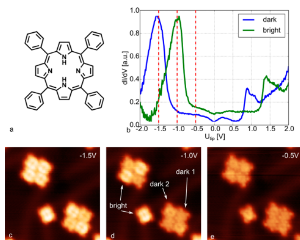
Figure 1. (a) Chemical structure of tetraphenylporphyrin (TPP). (b) dI/dV spectra of the dark and bright TPP molecules on Au(111). (c–e) STM images ( 11.4 \times 11.4 nm 2 , I_T = 0.44 nA, T = 5 K) of TPP on Au(111) with different tip bias voltages, which are indicated in the images and marked in (b) by red vertical lines.
