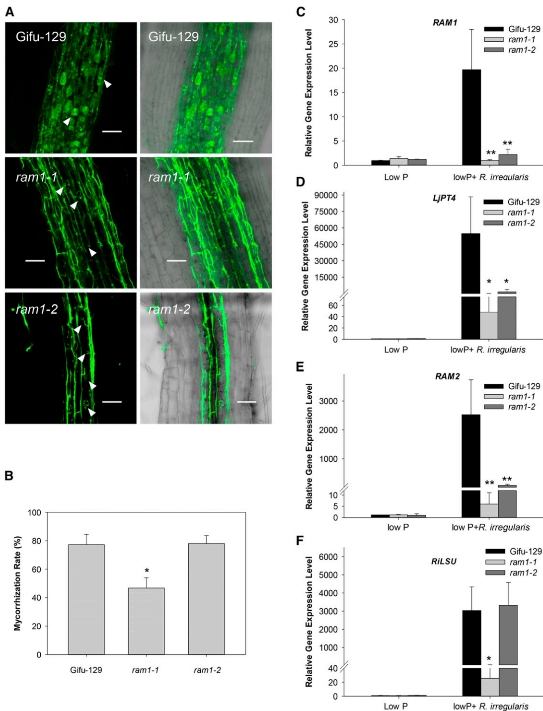
Figure 7. Mycorrhizal phenotype in two allelic RAM1 defective mutants. A , Gifu-129, ram1-1 , and ram1-2 were inoculated with R. irregularis for 6 weeks. Scale bars = 50 \mu m. Fungal structures were stained with Alexa Fluor 488. White arrows indicate arbuscules. B , Mycorrhization rate in Gifu-129 and ram1 alleles. Four biological replicates were used. Error bars represent SD ( n = 4 ). Student's t test was used between Gifu-129 and the two ram1 alleles. Asterisks indicate P < 0.05 . C to F , Mycorrhizal marker gene expression in wild-type and ram1 alleles. Mean values ( \pm SD) of four biological replicates are presented. Student's t test was used. Asterisks indicate significant difference relative to wild-type Gifu-129. * P < 0.05 ; ** P < 0.01 .
